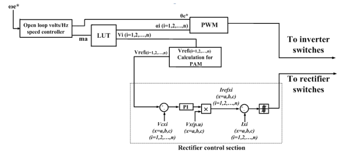
Fig. 7. Control block diagram of Fig. 1.
