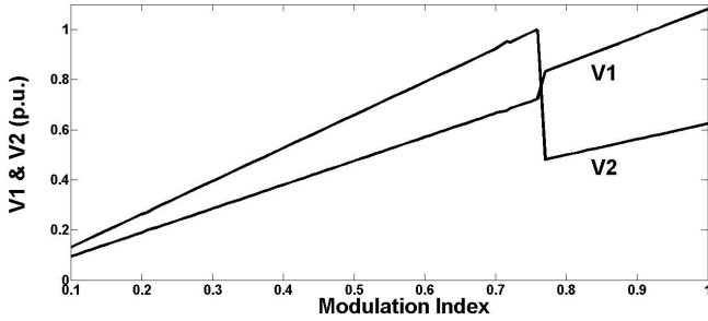
Fig. 4. V_1 and V_2 voltage values versus m_a in SHE-PWAM.
