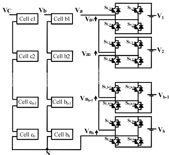
Fig. 1. The three phase CHB inverter topology.
