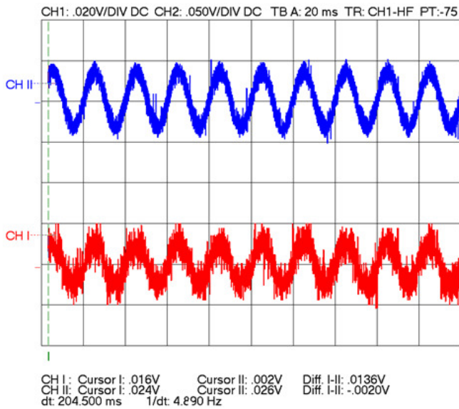
Fig. 9. Experimental input voltage and current of phase A.
