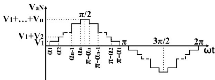
Fig. 2. Low frequency multilevel output voltage.
