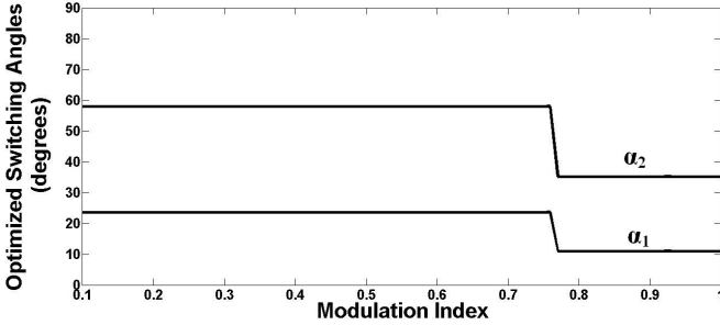
Fig. 5. Optimized switching angles versus m_a in SHE-PWAM.
