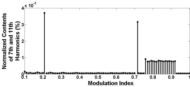
Fig. 6. Normalized contents of the 7 th and 11 th harmonics in SHE-PWAM.
