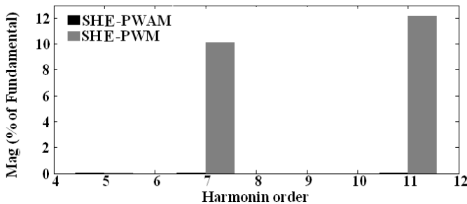
Fig. 11. 5th, 7th and 11th harmonics magnitude in both cases.
