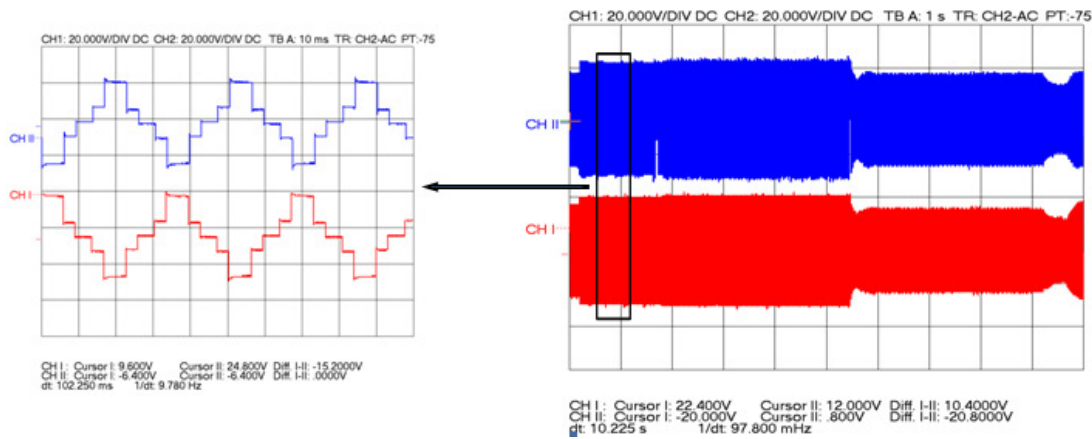
Fig. 8. Experimental V_{an} and V_{bn} phase voltages.
