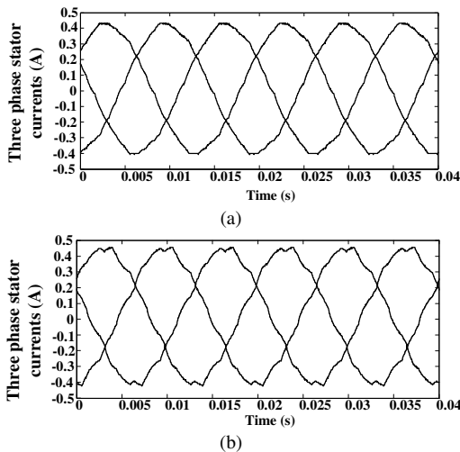
Fig. 10. Experimental stator three-phase currents after applying the nominal torque at rated speed and frequency a) SHE-PWAM b) SHE-PWM.
