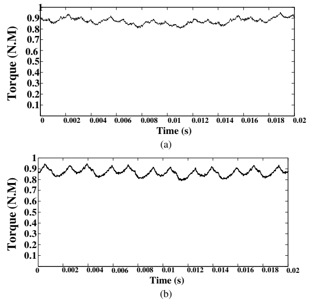
Fig. 12. Experimental torque a) SHE-PWAM b)SHE-PWM.
