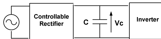
Fig. 3. Use of controllable rectifiers realizing variable dc sources.
