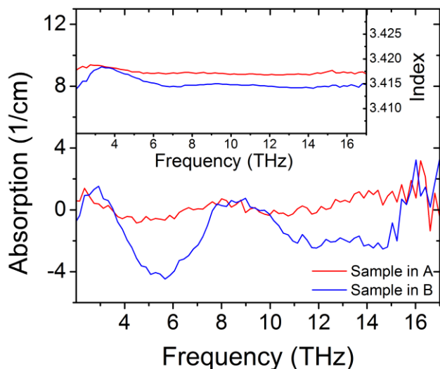
Fig. 3: Frequency dependent absorption coefficient and index of refraction of silicon in the case the sample is positioned in the collimated section of the THz beam (A) and in the focal point (B) of the spectrometer.
