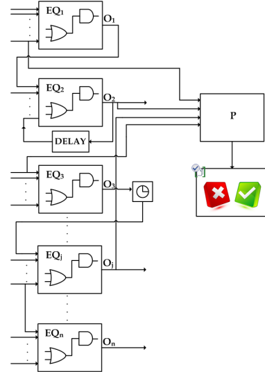
Figure 4. Prove Property
