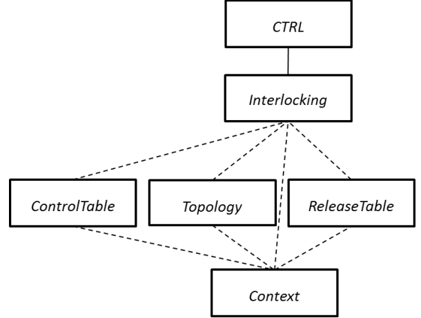
Fig. 2. CSP||B Architecture.
