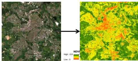
Figure 2. (left) Landsat true colour image June 2013, (right) MVC NDVI May-July 2013
