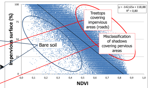
Figure 5. OLS regression impermeious surface and NDVI, City of Odense, Denmark
