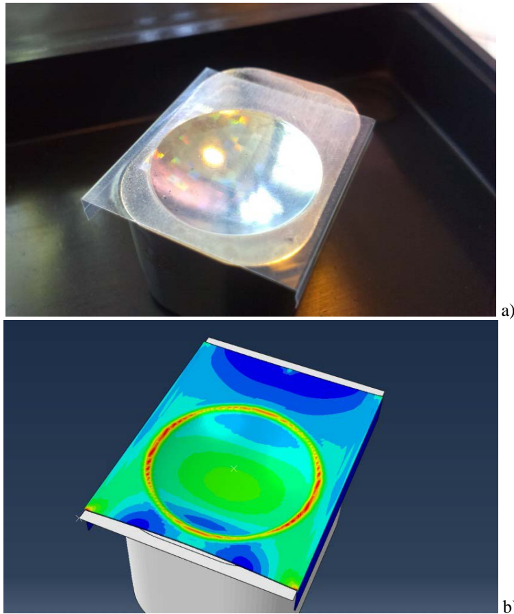
FIG. 2: NIL on the double-curved tool insert for injection moulding. In this case, the mould consists of a hemisphere with a radius of 15 mm and a height of 3 mm. a) The used PTFE flexible stamp with the glitter-effect pattern, on top of the steel tool insert after nanoimprint. b) Numerical model of the same setup, where it is possible to study the stretch and deformation of the flexible stamp, in combination with the actual imprinting pressure underneath the flexible stamp.
