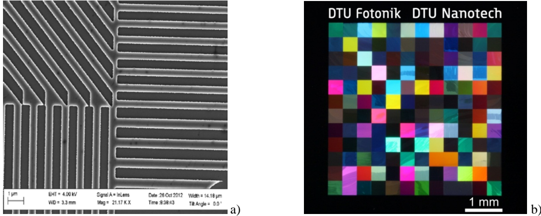
FIG. 1: By combining diffraction gratings with different periods and orientations a glitter-effect can be created. a) Close-up SEM image of the intersection between four different areas with different periods and orientations. b) Photo of glitter sample in black PMMA.
