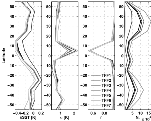
Figure 4. Latitude dependent statistics of the SE-VIRI-Drifter TFF.
