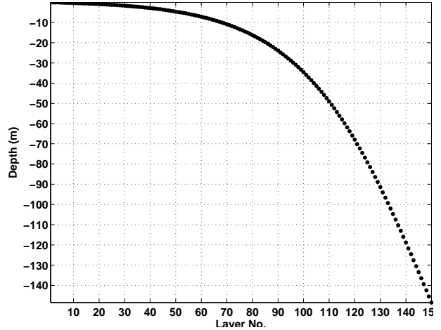
Figure 1. Distribution of GOTM vertical layers with depth.
