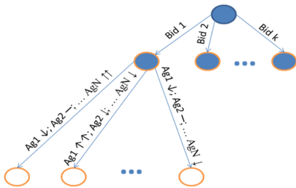
Fig. 2. Game theory for scenario-space search.
