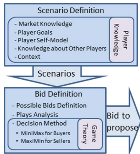
Fig. 1. Scenario Analysis Algorithm.
