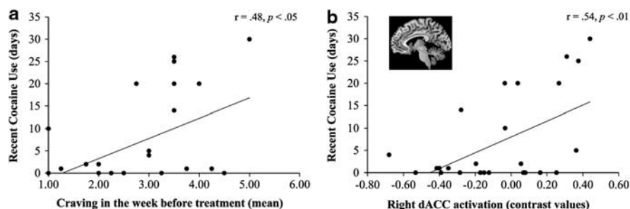
Figure 2 Correlation between (a) craving in the week before treatment and recent cocaine use and (b) attentional bias-related activation in the right dACC and recent cocaine use. dACC, dorsal anterior cingulate cortex.
