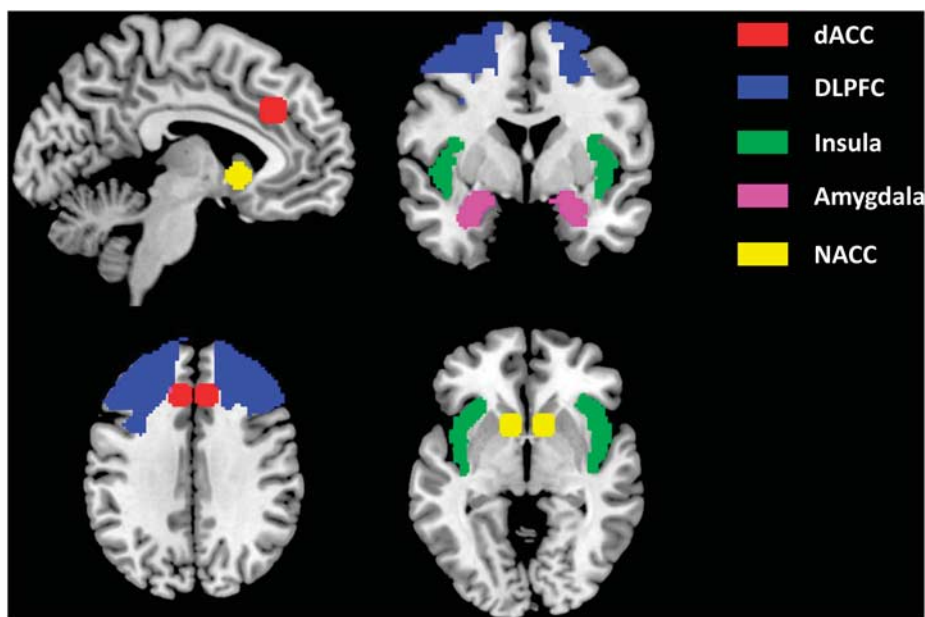
Figure 1 A priori defined, literature-based regions of interest involved in attentional bias to substance cues. dACC, dorsal anterior cingulate cortex; DLPFC, dorsolateral prefrontal cortex; NACC, nucleus accumbens.
