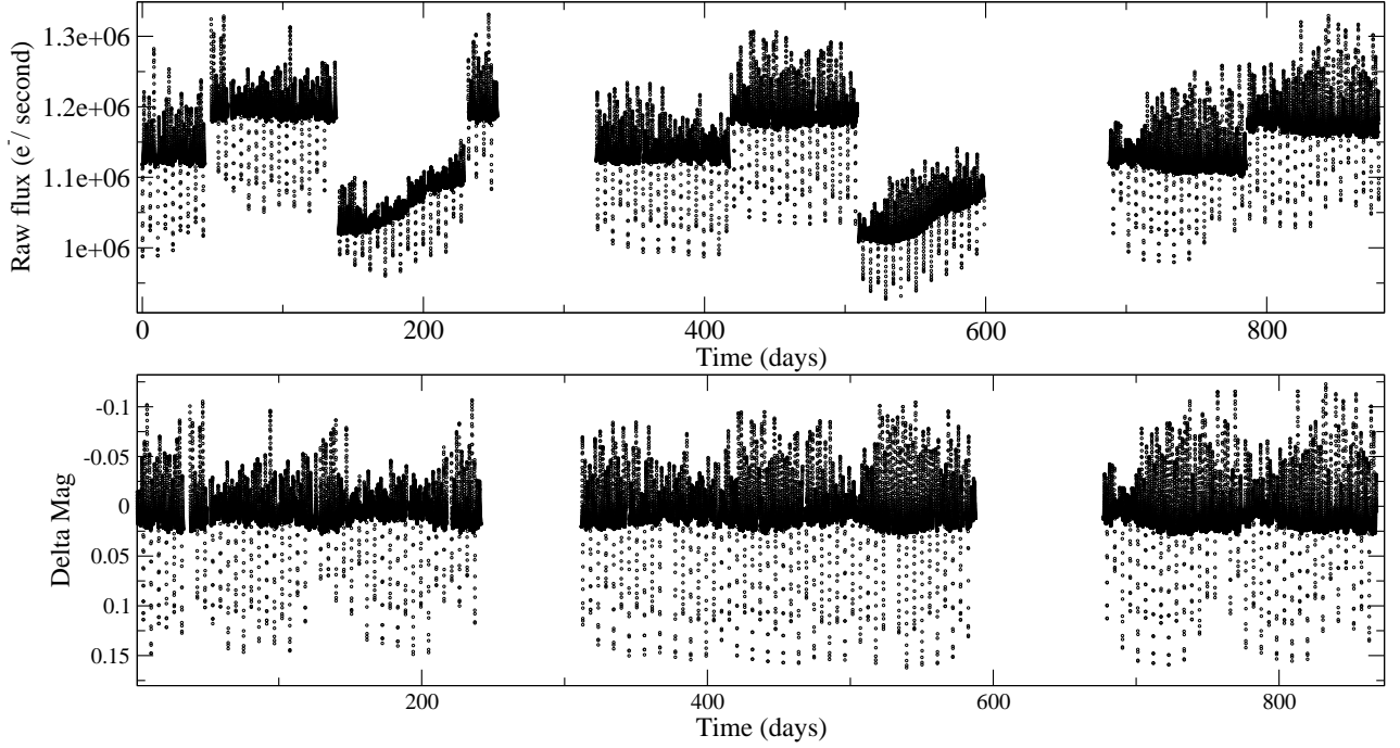
Figure 1. Combination of observing quarters Q1-Q10 for KIC 11285625. The top panel shows the ‘raw’ SAP (simple aperture photometry) fluxes, as they were delivered, while the lower panel shows the resulting combined dataset after optimal mask selection and detrending.
