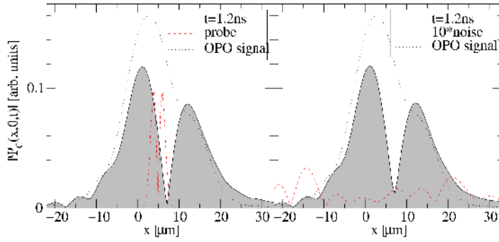
Fig. 9 Steady state filtered signal profile (dotted line) |\psi_c(x,0,t)| for y=0 before the arrival of either a Laguerre-Gauss vortex probe (24) with \omega_{\text{probe}}=1\text{tm} (left panel, red dashed line) or a noise pulse of strength 0.01 (right panel, red dashed line) — same OPO conditions as Fig. 8. After the arrival of any perturbation breaking the y \rightarrow -y symmetry, the same vortex with charge m = \pm 1 (solid shaded curve) stabilises into the signal. [From [22] ask for copyright permission!]
