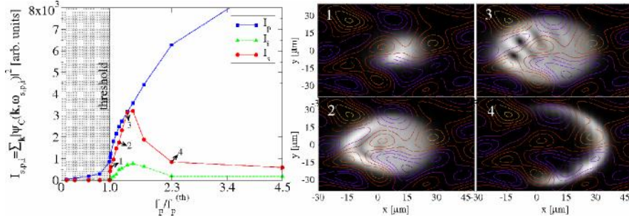
Fig. 6 Evolution of the signal, idler and pump state intensities as a function of the pump intensity f_p/f_p^{\text{th}} (left). Space profiles of the filtered signal at different values of the pump intensity (right). The parameters are the same as in Fig. 4, with the addition of a photonic disorder potential V_C(\mathbf{r}) , correlation length L_d 20 \mu\text{m} and strength \sigma_d 0.1 meV (contour-level lines in the panels on the right).
