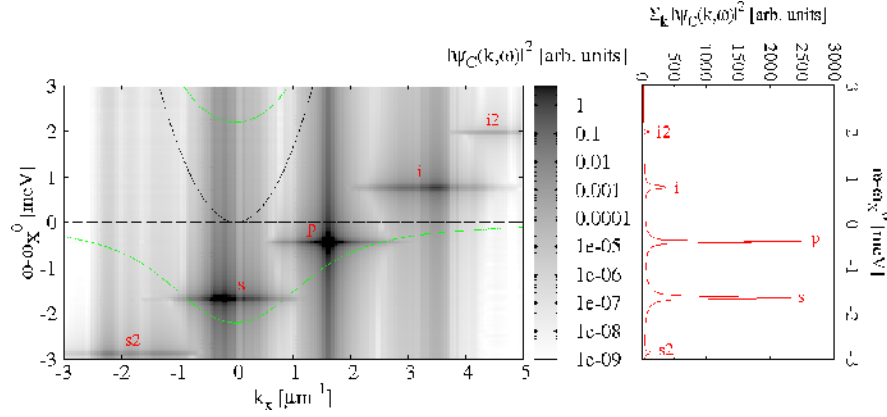
Fig. 4 Left panel: OPO spectrum |W_{C,X}(k, \omega)|^2 for a top-hat pump of FWHM a_p = 70 \text{ Åm} and intensity f_p = 1.25f_p^{\text{th}} above the threshold pump power for OPO, f_p^{\text{th}} . For this particular run we resonantly pump at k_p = 1.6 \text{ Åm}^{-1} in the X -direction, \mathbf{k}_p = (k_p, 0) , and at \omega_p - \omega_x^0 = -0.44 \text{ meV} . Polaritons at the pump state undergo coherent stimulated scattering into the signal and idler states, which are blue-shifted with respect to the bare lower polariton (LP) dispersion (green dotted line) because of interactions. Cavity photon (C) and exciton (X) dispersions are plotted as gray dotted lines. Above threshold, as discussed in the text, we observe the population of the satellite states in addition to the one of signal and idler. Right panel: Momentum integrated spectrum, \sum_k |W_{C,X}(k, \omega)|^2 , as a function of the rescaled energy \omega - \omega_x^0 . Pump, signal, idler and satellite states are all equally spaced in energy by roughly 1.19 meV.
