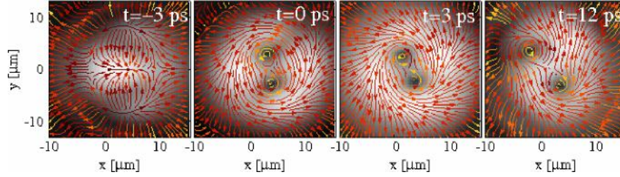
Fig. 16 Filtered signal profile and currents above threshold for OPO ( f_p = 1.12f_{th} ) for a top-hat pump with FWHM \sigma_p = 35 \mu\text{m} at t = -3 \text{ ps} (first panel) before the arrival of an m = 2 probe. The doubly quantised vortex gets transferred from the probe into the OPO signal and splits into two m = 1 vortices even before the probe reaches its maximum intensity at t = 0 \text{ ps} (second panel). In this simulation the vortices coexist for sometime (roughly 15 ps), then one gets expelled from the signal (fourth panel). Adapted from [23].
