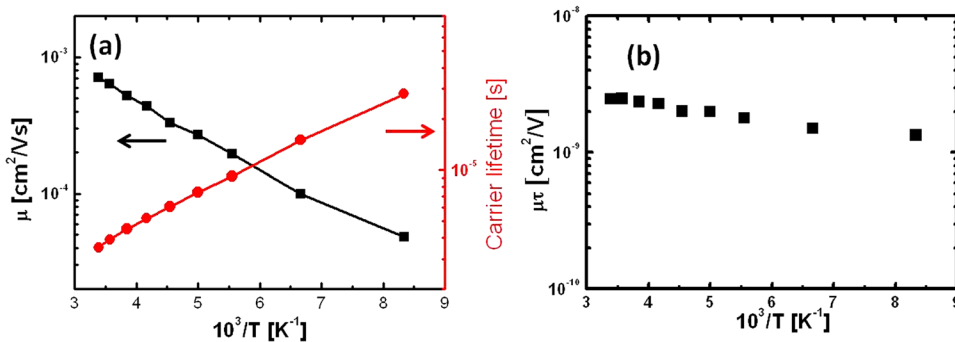
FIG. 5. (a) Charge carrier half-decay lifetime measured from concentration decay (shown in Figure 4(b)) and charge mobility (shown in Figure 3(a)) and (b) shows mobility-lifetime product \mu\tau_{\beta} in the range of studied temperatures. Temperature independent \mu\tau_{\beta} product shows that reduction in charge carrier mobility results in longer carrier lifetime, as expected in Langevin-type bimolecular recombination, where the recombination rate is determined by their movement velocity (charge mobility).
