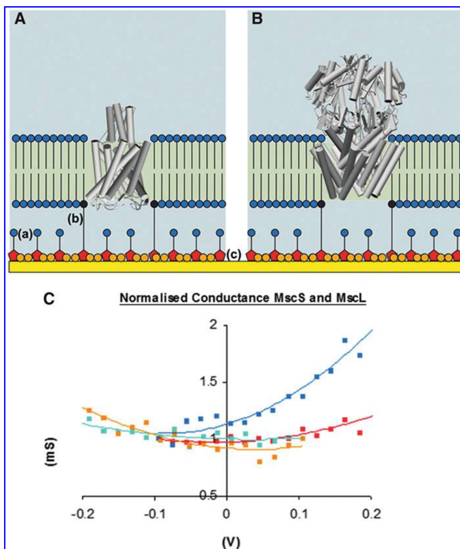
FIG. 6. Electrical recording of MscL and MscS activity in tethered bilayers. Schematic of a tethered lipid bilayer containing (A) MscL and (B) MscS. Short hydrophilic spacer molecules (a) are interspersed with tethers (b) that anchor the lipid bilayer by penetrating the monolayer leaflet of the bilayer. The hydrophilic segment of the tether molecules is twice the length of the hydrophilic segment of the spacers. This is intended to permit accommodation of segments of the MscL or MscS that may protrude beyond the inner leaflet of the bilayer toward the tethering gold surface. Both the spacers and the lipid tethers are anchored to a gold electrode by sulfide chemistry (c). The region between the gold surface and the tethered lipid bilayer membrane forms an ionic reservoir permitting measurement of ion fluxes that pass through the membrane. The tethering sulfur groups also include a phenyl disulphide moiety that provides space between the tethers and spacers to facilitate ionic diffusion within the reservoir space. MscL and MscS can be reconstituted into the tethered bilayer, and impedance spectroscopy can then be used to measure the conductance across the membrane caused by the presence of the channels. (C) Normalized conductance–voltage relationship for MscS and MscL reconstituted into tethered bilayers. In C20 diphytanyl (70%) hydroxyglycerol (30%) tethered membranes: MscS conductance is voltage dependent and rectifying in the range +100 to –200 mV (cyan squares) and –100 to +200 mV (blue squares); MscL is essentially independent of voltage over the same range of +100 to –200 mV (gold squares) and –100 to +200 mV (red squares); Note that polarity is defined by the gold electrode tethering the membrane relative to the counter electrode. In the inner leaflet, 10% of the lipids were tethers and 90% were mobile. In the outer leaflet, all lipids were mobile. At the gold surface, the spacer groups are ~2 nm in length, and the thickness of the reservoir space between the gold and the inner surface of the membrane was ~4 nm in length. To see this illustration in color, the reader is referred to the web version of this article at www.liebertpub.com/ars
