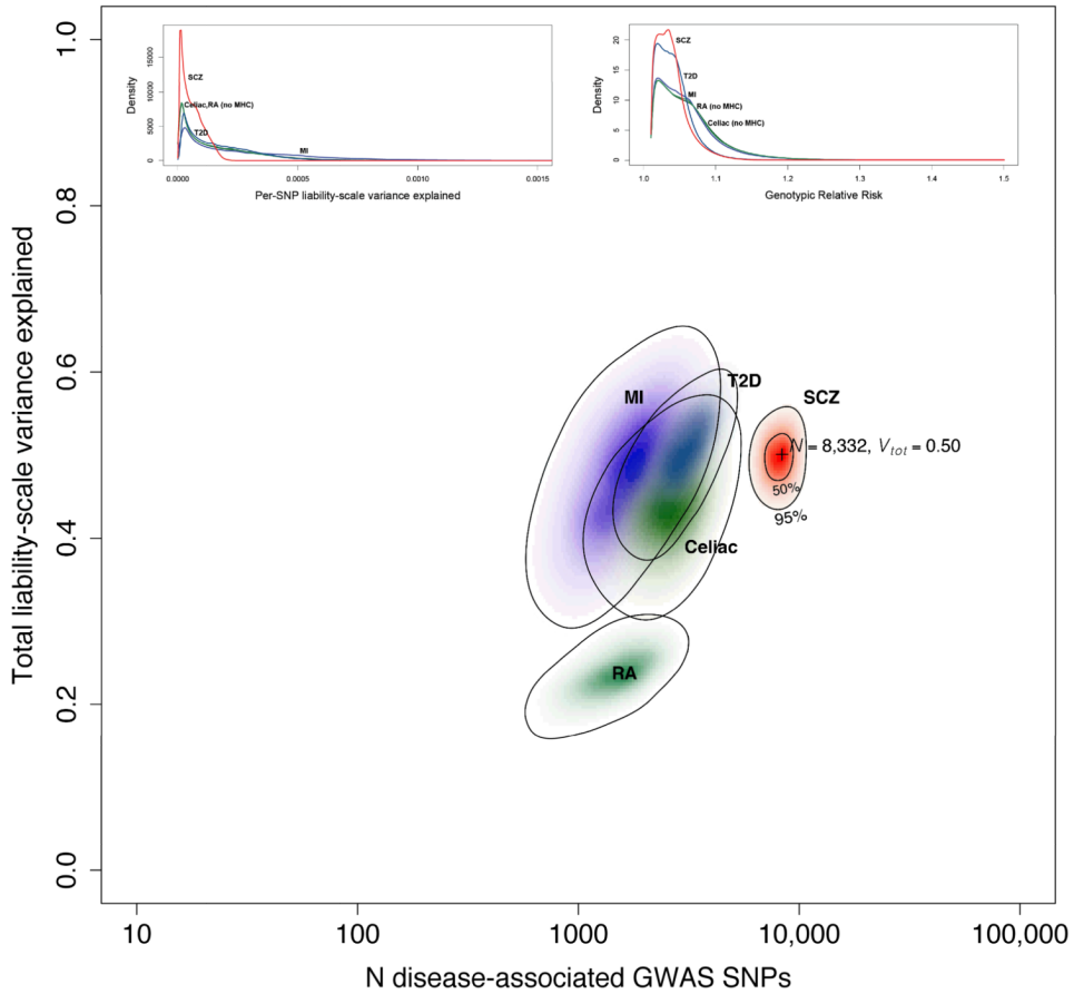
Figure 3. The main figure shows the results of ABPA modeling based on the Sweden + PGC results (population risk 0.01). The x-axis is the estimated number of SNPs on a \log_{10} scale, and the y-axis estimates the total variance in liability explained. The results for five conditions are shown: schizophrenia (this analysis, red) and, for comparison, results from a published analysis of myocardial infarction (MI, purple), type 2 diabetes mellitus (T2D, blue), celiac disease (green), and rheumatoid arthritis (RA, teal). 71 The schizophrenia results are based on 1000 Genomes imputation, and the others on HapMap3 imputation. Color intensity reflects the probability density with darker colors indicating higher density. Contour lines show 50% and 95% credible regions for SCZ, and 95% credible regions for the other diseases. The insets depict estimated SNP distributions for the five disorders: (a) distribution of SNPs in terms of the variance in liability explained per SNP and (b) the estimated distribution of SNP genotypic relative risks (GRR). We again stress that multiple qualifiers are essential in interpreting these estimates.
