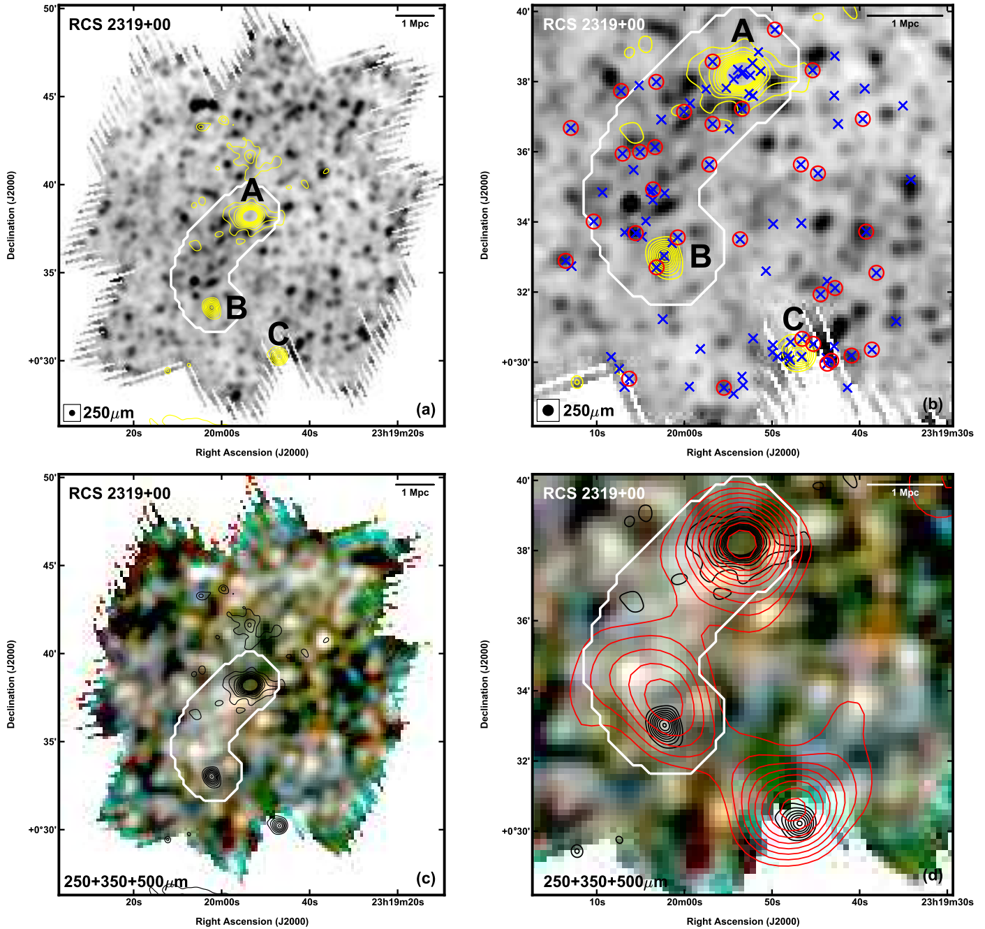
FIG. 1.— The Herschel filament in RCS 2319+00. The white outline indicates the filamentary region defined for the analysis, spanning components A–B, and is overlaid on the 250\ \mu\text{m} SPIRE map ( panels a and b ) and on an RGB composite of the 250 , 350 and 500\ \mu\text{m} maps smoothed to the lowest resolution ( panels c and d ). Smoothed X-ray emission contours (with the point-sources removed) are overplotted in yellow ( panels a and b ) or in black ( panels c and d ). Panel b ) Blue ‘x’ symbols indicate the positions of the 41 confirmed 0.8700 < z < 0.9247 cluster members, and are encircled in red if they are 24\ \mu\text{m} -detected. Panel d ) The red contours trace the surface density of galaxies selected by the RCS selection of ‘red-sequence’ galaxies at z \sim 0.9 . As pointed out in Gilbank et al. (2008b), note that the major axis of the red-sequence clusters tends to point towards its nearest neighbour, and also notice the striking offset from the red-sequence defined cluster cores ‘B’ and ‘C’ to the peaks of the X-ray emission.
