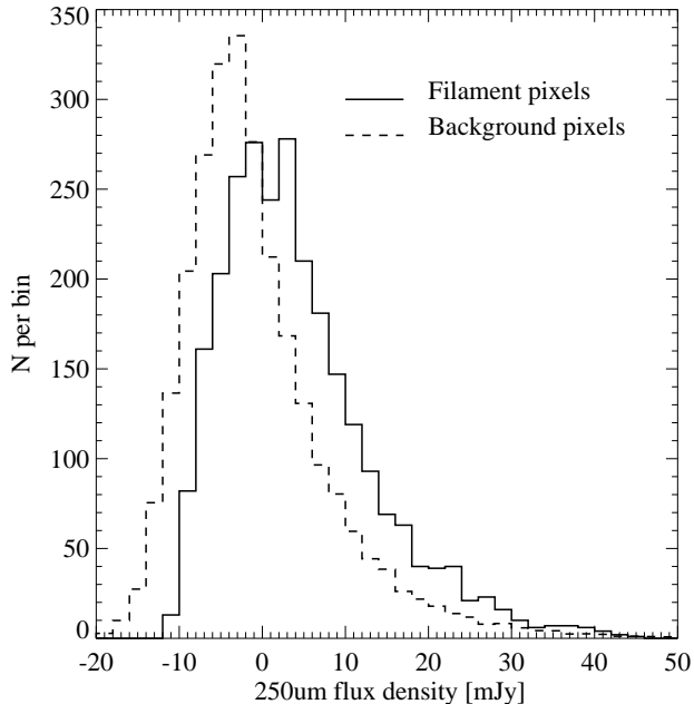
FIG. 2.— Area-normalized 250 \mu\text{m} pixel flux histograms showing a striking excess of far-IR emission in the filament versus the background (pixels outside the filament region).
