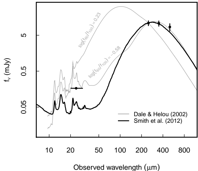
FIG. 3.— SEDs redshifted to z = 0.9 and normalized to the average (stacked) 250 \mu\text{m} SPIRE flux at the 14 24 \mu\text{m} cluster members in the filament. Three SED templates have been plotted for illustrative purposes, including the two extremes of the Dale & Helou (2002) library (in terms of the S_{60}/S_{100} color), as well as the Smith et al. (2012) H-ATLAS galaxy template with 1 \times 10^{11} L_{\odot} < L_{\text{dust}} < 3 \times 10^{11} L_{\odot} . The ‘cool’ color SED templates from Dale & Helou (2002), as well as the H-ATLAS SED are well matched to the average far-IR emission of MIPS-selected emitters in the filament. At z = 0.9 , the 24 \mu\text{m} band is tracing the rest-frame 13 \mu\text{m} light, which is dominated by a complex of broad PAH emission, thus we expect some variation in SED template matches in this band, as is seen here.
