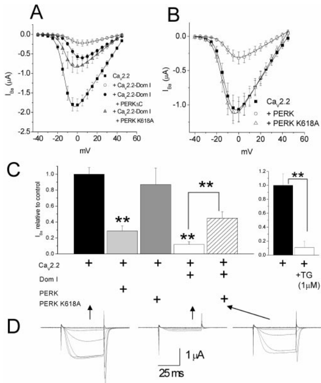
Figure 1. The effect of PERK and dominant-negative PERK constructs on suppression of \text{Ca}_v2.2 I_{Ba} by \text{Ca}_v2.2\text{-Dom I} , \text{Ca}_v2.2/\alpha2\delta-2/\beta1b I_{Ba} recorded in Xenopus oocytes, either in the absence (■; n = 29 ) or presence of \text{Ca}_v2.2\text{-Dom I} (○; n = 19 ), \text{Ca}_v2.2\text{-Dom I} plus PERK K618A (△; n = 24 ), or \text{Ca}_v2.2\text{-Dom I} plus PERK ΔC (●; n = 18 ). The mean I - V plots gave maximum conductance ( G_{max} ) values of 38.6, 6.1, 19.4, and 15.4 \mu\text{S} , respectively. B , \text{Ca}_v2.2/\alpha2\delta-2/\beta1b I_{Ba} recorded in the same experiments either in the absence (■; n = 20 ) or presence of PERK (○; n = 15 ) or PERK K618A (△; n = 26 ). The mean I - V plots gave G_{max} values of 24.7, 9.4, and 27.0 \mu\text{S} , respectively. C , Left, Histogram of all mean data obtained at 0 mV for control \text{Ca}_v2.2/\beta1b/\alpha2\delta-2 I_{Ba} (■; n = 35 ) in the presence of PERK (□; n = 24 ), PERK K618A (▣; n = 26 ), \text{Ca}_v2.2\text{-Dom I} (□; n = 26 ) or \text{Ca}_v2.2\text{-Dom I} plus PERK K618A (▨; n = 27 ). Right, Effect of incubation of oocytes with thapsigargin (TG; 1 \mu\text{M} ; n = 3 ; □) compared with control (incubated with the same concentration of DMSO; ■; n = 10 ). Only 3 of 10 thapsigargin-treated oocytes showed any current compared with 10 of 11 control oocytes that expressed \text{Ca}_v2.2 currents in the same experiment. The mean peak I_{Ba} at 0 mV is expressed relative to control. Statistical significance compared with control or \text{Ca}_v2.2\text{-Dom I} where indicated: *** p < 0.001 . D , Examples of I_{Ba} : left, \text{Ca}_v2.2/\beta1b/\alpha2\delta-2 ; center, plus \text{Ca}_v2.2\text{-Dom I} ; right, plus \text{Ca}_v2.2\text{-Dom I} and PERK K618A. The calibration bar refers to all panels. I_{Ba} is shown in 5 mV steps between -40 and 0 mV.
