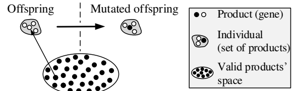
Figure 4: Mutation operation. A random product is selected from the offspring and replaced by a product randomly selected from the space of all the products valid towards the Feature Model.
