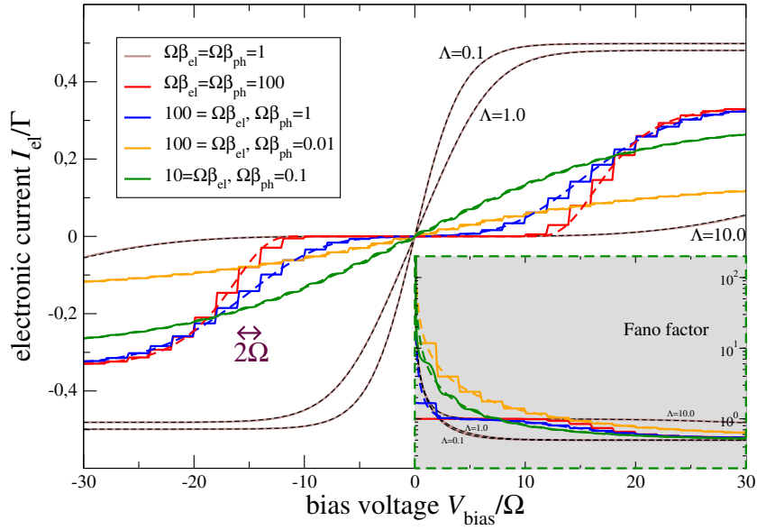
Figure 3. The electronic current and Fano factor (inset) for the single-mode (solid) and continuum (dashed) cases for different temperature configurations (colored curves) and different coupling strengths (brown solid and black dashed). Low electronic temperatures are required for resolving the single-mode nature of the phonon bath (step-like solid curves versus smooth dashed curves). The reduction of even the large-bias currents is a consequence of a constant and finite width of the electronic tunneling rates. Other parameters: \Gamma_L = \Gamma_R = \Gamma , \delta = 10\Omega , \epsilon/\Omega = 0 , \Omega = \omega_c , and for the bold colored curves \Lambda = |\hbar|^2/\Omega^2 = J_0 = 5 .
