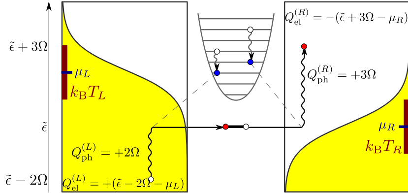
Figure 1. Sketch of the heat transfer energetics at the trajectory level for the single-phonon mode ( Q = 1 ) case and for two sample elementary processes (black solid with specific heat flows into the system noted). Filled regions left and right denote Fermi functions of left and right electronic leads, whereas the sketched oscillator denotes the phonon reservoir, respectively. During the electronic tunneling events (wavy lines), energy from the phonons may assist electrons far from the dot level \tilde{\epsilon} to participate in transport. In the left trajectory, an electron jumps from the left lead to the initially empty dot via the emission of two quanta by the phonons. In the right trajectory, it leaves the dot to the right lead via the emission of two quanta by the phonons. For trajectories with identical initial and final SET states (the change of SET entropy is zero), the total entropy production is minus the entropy flow and is given by \Delta_i S = -Q_{\text{el}}^{(L)}/T_L - Q_{\text{el}}^{(R)}/T_R - (Q_{\text{ph}}^{(L)} + Q_{\text{ph}}^{(R)})/T_{\text{ph}} , with transferred electronic heat Q_{\text{el}}^{(\alpha)} = -(\tilde{\epsilon}n_{\text{el}}^{(\alpha)} - e_{\text{ph}}^{(\alpha)} + \mu_{\alpha}n_{\text{el}}^{(\alpha)}) and the associated phonon heat Q_{\text{ph}}^{(\alpha)} = -e_{\text{ph}}^{(\alpha)} . For example, the combination of both trajectories shown yields with n_{\text{el}}^{(L)} = -1 , n_{\text{el}}^{(R)} = +1 , e_{\text{ph}}^{(L)} = -2\Omega , and e_{\text{ph}}^{(R)} = -3\Omega altogether a total entropy production of \Delta_i S = -(\tilde{\epsilon} - 2\Omega - \mu_L)/T_L - 5\Omega/T_{\text{ph}} + (\tilde{\epsilon} + 3\Omega - \mu_R)/T_R .
