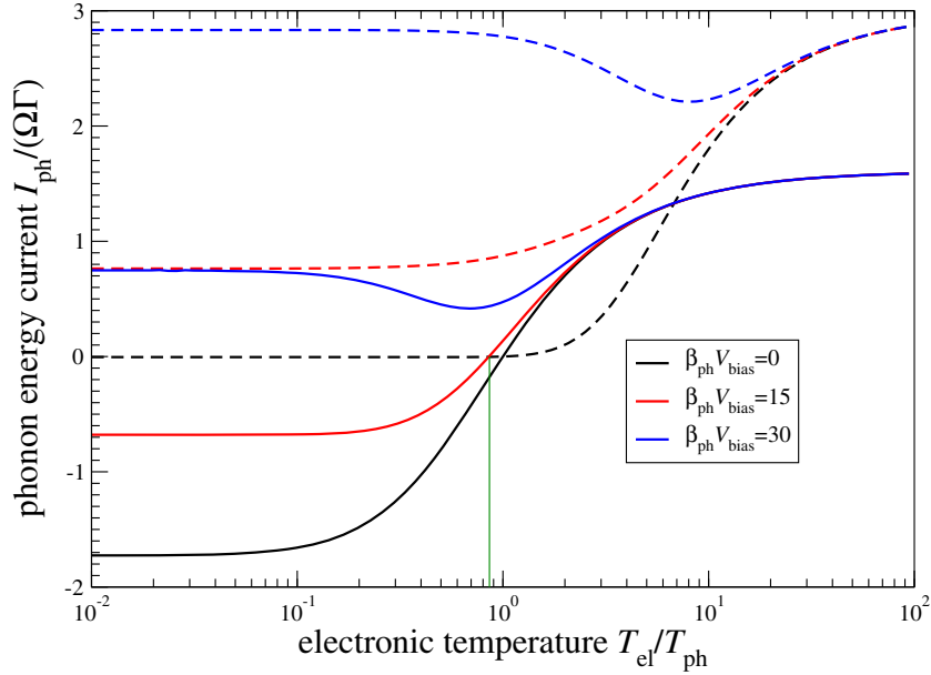
Figure 4. The total energy current into the phonon bath versus electronic temperature T_{\text{el}}/T_{\text{ph}} for different phonon temperatures \beta_{\text{ph}}\Omega = 0.1 (solid), \beta_{\text{ph}}\Omega = 1.0 (dashed) and vanishing V_{\text{bias}}\Omega = 0 (black), intermediate V_{\text{bias}}\Omega = 15 (red) and high V_{\text{bias}}\Omega = 30 (blue) electronic bias voltages. Other parameters: \Gamma_{\text{L}} = \Gamma_{\text{R}} , \delta = 10\Omega , \epsilon/\Omega = 0 , \Omega\beta_{\text{ph}} = 1 , |h|^2/\Omega^2 = 5 .
