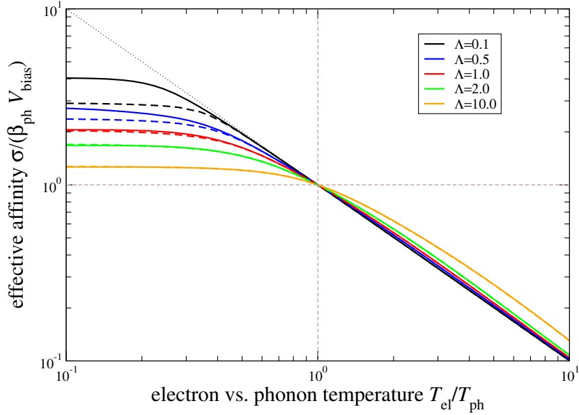
Figure 2. Effective affinity \sigma , equation (10), for different values of the coupling strength \Lambda = |\hbar|^2 / \Omega^2 in the single-mode case (solid lines) or \Lambda = J_0 in the continuum case (dashed curves). When T_{\text{el}} = T_{\text{ph}} , the FT is independent of the coupling strength (intersection point). For vanishing coupling strength, we recover \sigma = \beta_{\text{el}}(\mu_{\text{L}} - \mu_{\text{R}}) (dotted thin curve). Other parameters: \Gamma_{\text{L}} = \Gamma_{\text{R}} , \beta_{\text{ph}}\mu_{\text{L}} = +5 , \beta_{\text{ph}}\mu_{\text{R}} = -5 , \delta = 10\Omega , \beta_{\text{ph}}\epsilon = 0 , and \beta_{\text{ph}}\Omega = \beta_{\text{ph}}\omega_{\text{c}} = 1 .
