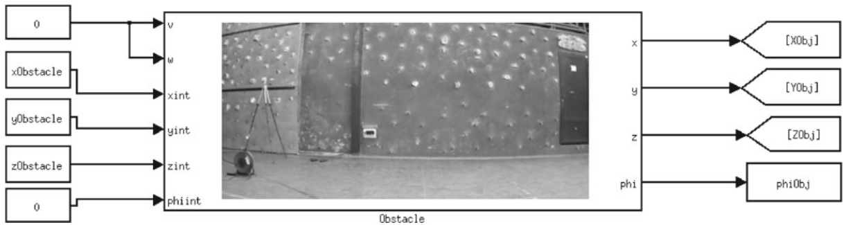
Fig. 11 Obstacle block in Matlab Simulink, where, the wall as the obstacle is tested
