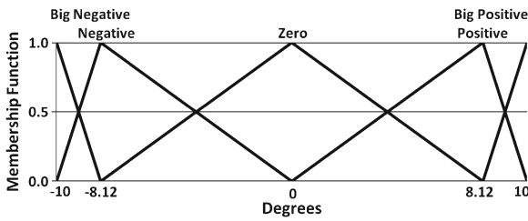
Fig. 27 Membership functions for Second input (Derivative of Yaw Error), after CE optimization, where, the Negative ( Positive ) has been optimized to -8.1166 ( 8.1166 )
