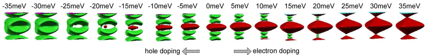
FIG. 11. (Color online) The Fermi surface of doped graphite in the dilute limit for electron doping and hole doping. The red (green) surfaces are the electron (hole) pockets of the Fermi surface. It is clear that at \pm 25 meV we have a semimetal to metal transition.
