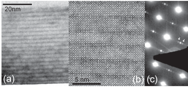
FIG. 1. Cross-sectional TEM images of a 20 bilayer \text{PbTiO}_3/\text{SrTiO}_3 3/3 sample. (a) Bright field image clearly shows the intended layering of the structure. (b) HRTEM shows the perfect crystalline structure of the material. (c) Diffraction image demonstrating superlattice periodicity.
