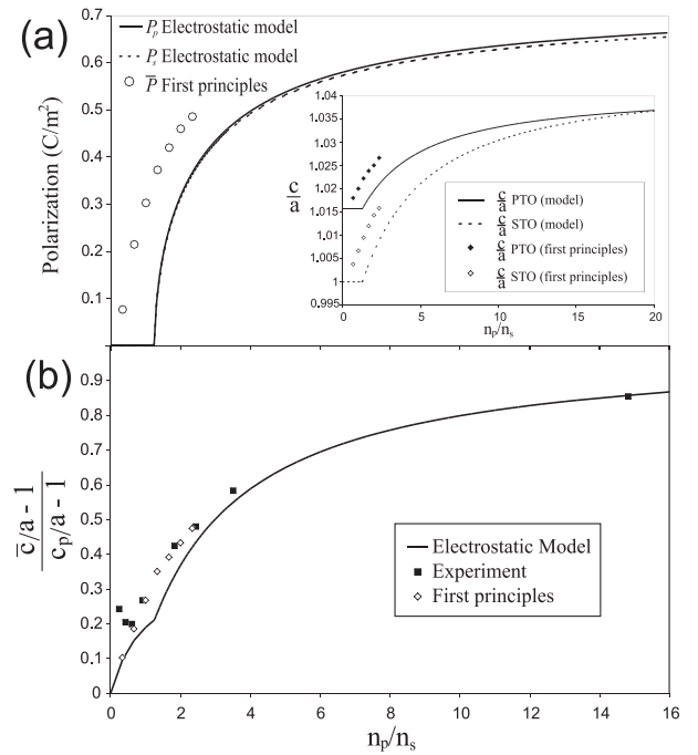
FIG. 4. (a) Polarization in each layer from the electrostatic model (dotted and solid lines) and the average polarization from first principles calculations (open circles). Inset shows tetragonality in each material calculated from both methods. (b) Comparison of experiment and both theoretical approaches.
