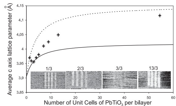
FIG. 3. Average c -axis lattice parameter plotted against the number of unit cells of lead titanate per bilayer showing the suppression and recovery of ferroelectricity. Complementary PFM images are shown as insets.
