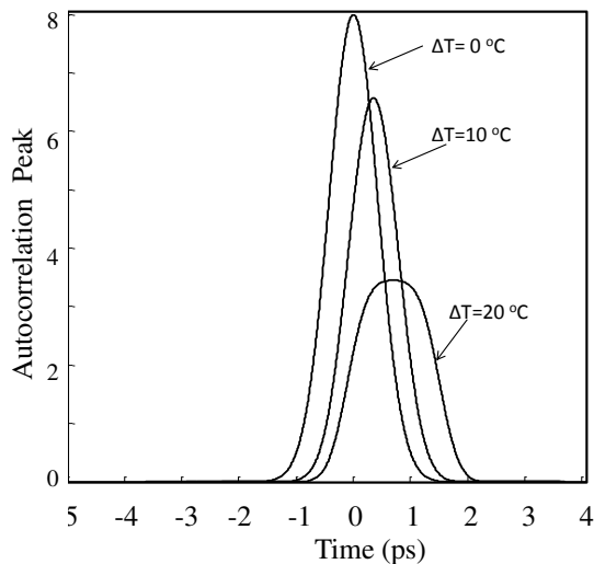
Fig.3 Maximum obtainable autocorrelation peak for different values of \Delta T at a link span of 10km
