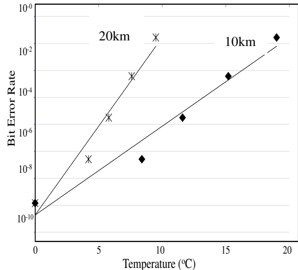
Fig.4 Minimum obtainable Bit Error Rate as \Delta T increases over a 10km link.
