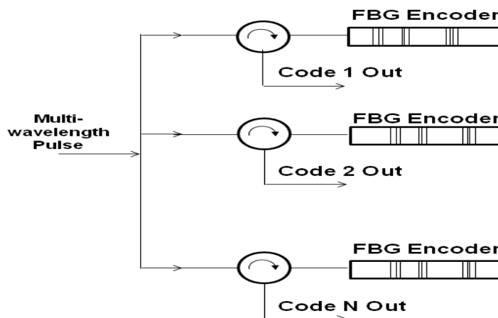
Fig. 1. Traditional method of generating OCDMA signals from a multiwavelength pulse
