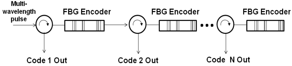
Fig. 2. Proposed cascade method that enables effective utilization of optical power
