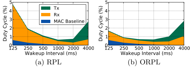
Figure 7: Energy Profiles (Upwards Routing). RPL and ORPL have different optima, because of a different balance between reception and transmission.
