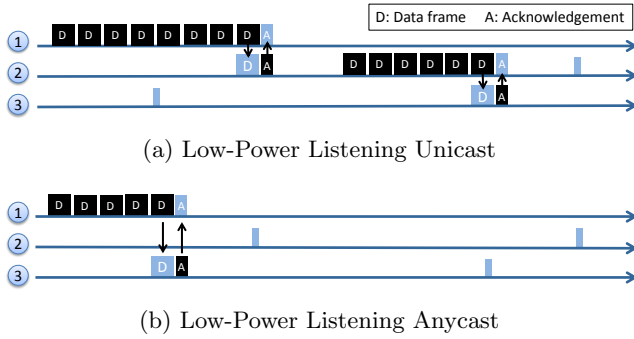
Figure 2: Traditionally, routing uses unicast over stable links, aiming for stability. Low-power listening introduces a significant delay at every hop. ORPL uses anycast and transmits to the first awoken forwarder that receives the packet, regardless of link quality estimates.
