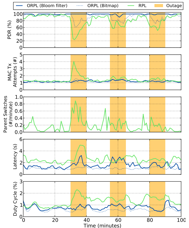
Figure 14: Robustness. ORPL maintains a reliability close to 100% during outages, partially through its recovery mechanism. RPL adjusts to topology changes, but loses data in the process.
