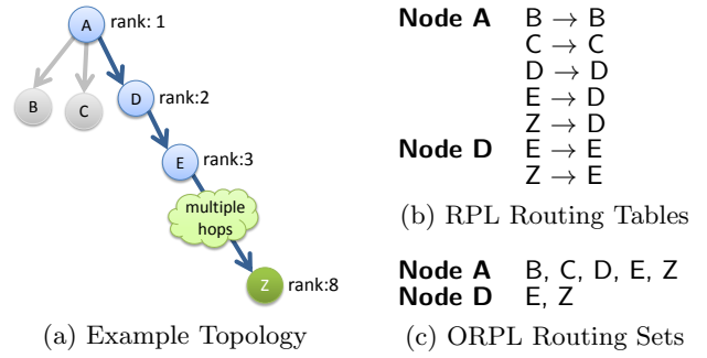
Figure 3: To reach Z, A has to route downwards with D as a next hop. In RPL, A uses a routing table and unicasts to D. In ORPL, D elects itself as next hop upon receiving A’s anycast, based on the inclusion of Z in its own routing set and on the increasing rank.
