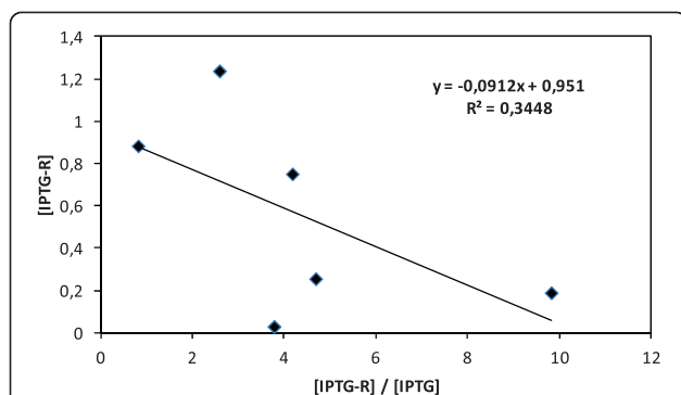
Figure 6 Bound inducer concentration (calculated as inducer missing concentration) vs. the ratio between bound inducer concentration/measured inducer concentrations. The slope corresponds to -1/K_c . The intercept corresponds to total repressor concentration. The analytical standard error for experimental IPTG measurements is 5 and 7% for medium and intracellular samples, respectively.
