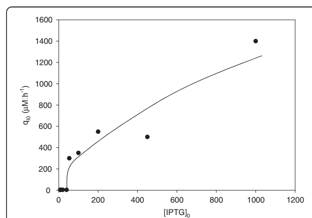
Figure 1 Initial IPTG transport rate ( q_{I0} , \mu\text{M}\cdot\text{h}^{-1} ) from medium to the biomass vs. initial inducer concentration ( \text{IPTG}_0 , \mu\text{M} ) in fed-batch substrate limiting experiments. Each point corresponds to the initial slope of IPTG medium concentration profile.
