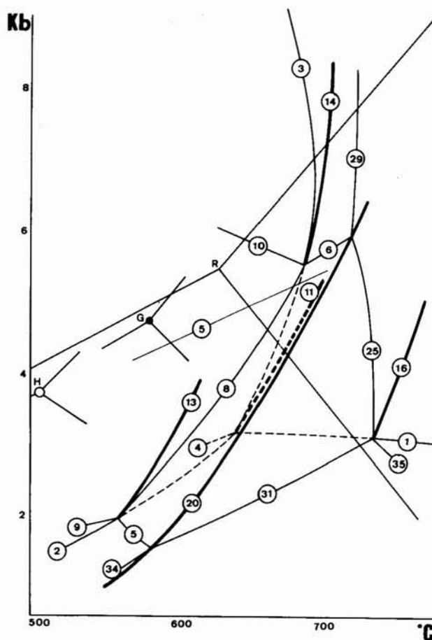
Fig. 6.—Semi-quantitative P-T projection of studied reactions for low- f_{O_2} (QFM buffer). P_{H_2O} = P_1 in metapelites with excess quartz, muscovite and water.
