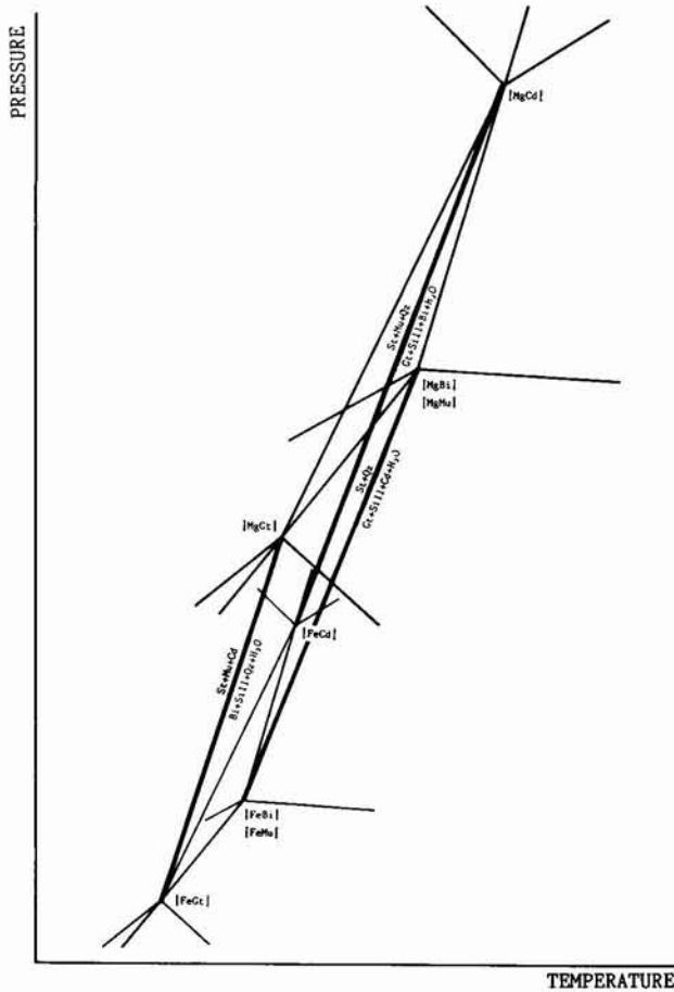
Fig. 3.—Schematic diagram of P-T-X Fe-Mg relationships between Gt-Cd-St-Bi-Mu-Als projected on the P-T plane. Systems KFASH-KMASH-KFMASH. Univariant reaction slopes taken from Table 3. Light line: Fe pole; regular line: Mg pole; Heavy line: KFMASH univariant reactions.
