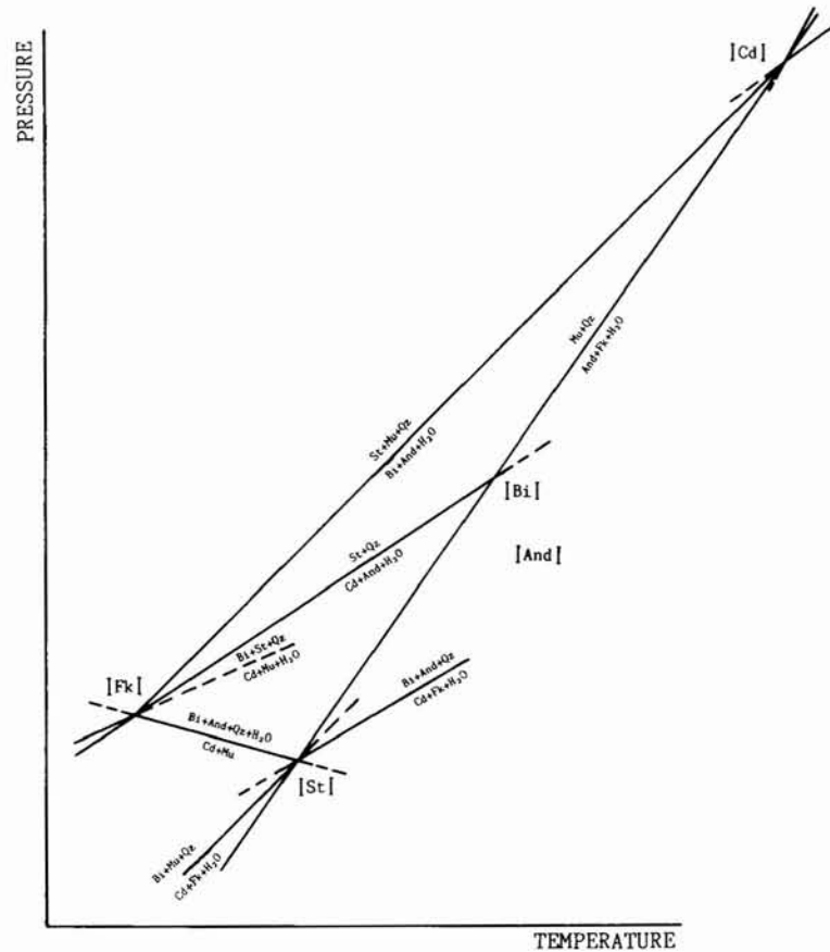
Fig. 5.—P-T arrangement of reactions between Cd-St-Bi-Mu-And-Fk (excess Qz and H 2 O) in KFASH system. Dashed lines are metastable extensions. Approximate slopes 1Kb/50°C.
