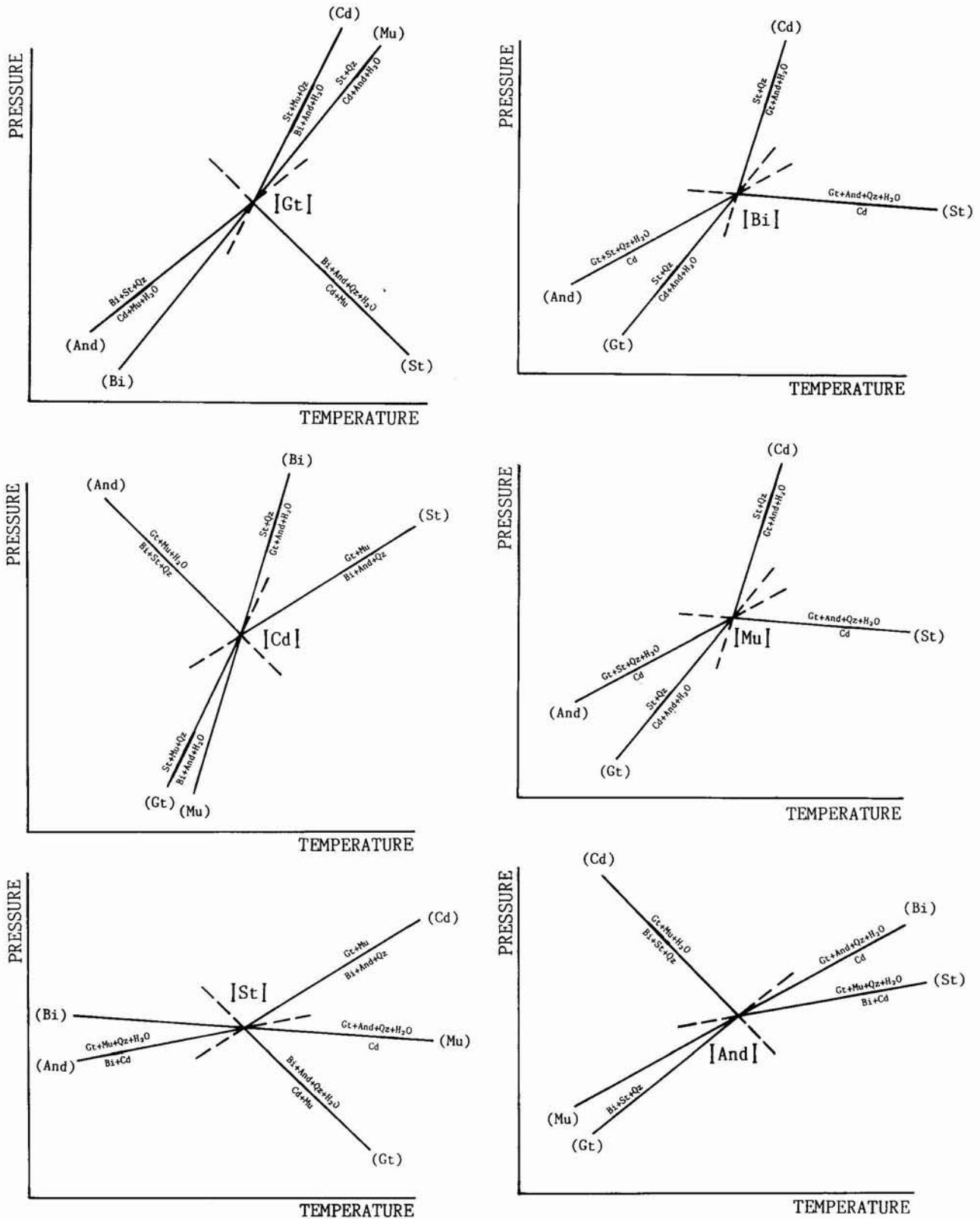
Fig. 1.—P-T arrangement of univariant equilibria and divariant fields around invariant points in KFSH system. Phases are Gt-Cd-St-Bi-Mu-And (excess Qtz and H 2 O). Dashed lines are metastable extensions of univariant equilibria. Approximate slopes 1Kb/100°C.
