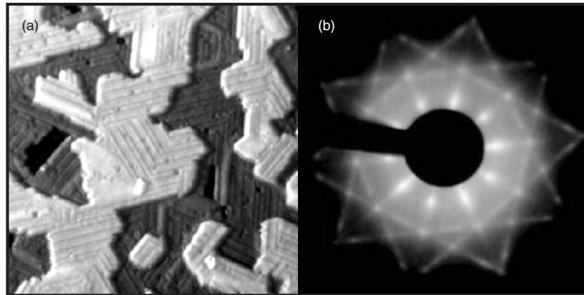
Figure 9. (a) 40\text{ nm} \times 40\text{ nm} STM image of 5.5 \pm 0.2\text{ ML} Cu adsorbed on the fivefold face of icosahedral Al–Pd–Mn. (b) A LEED pattern taken from this surface at 169 eV. Reprinted with permission from [100]. Copyright 2004, American Physical Society.
