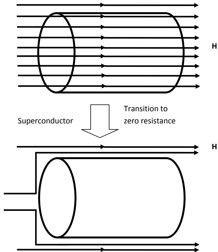
Figure 4: The magnetic flux completely expelled from its interior superconductor
