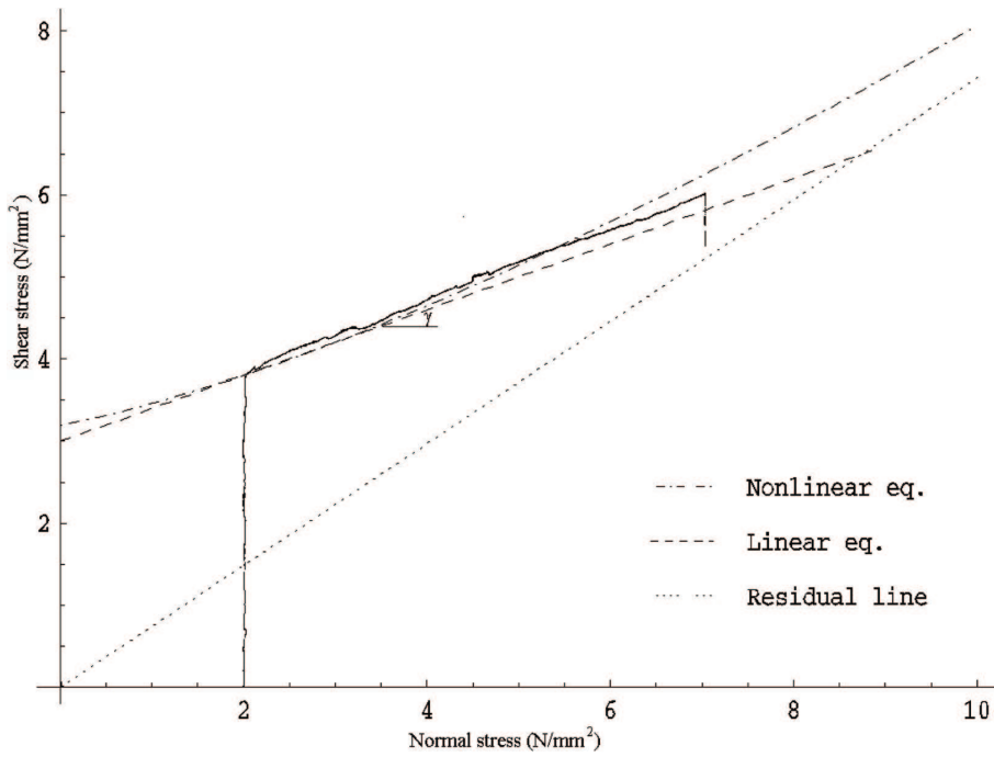
Fig. 6. Comparing the linear equation, the non-linear equation and the measured normal stress-shear stress curve in case of 2.0 N/mm 2 starting normal stress.
