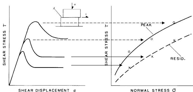
Fig. 1. Characteristic results of direct tests with constant normal loading on rock joints indicating similarity to triaxial test results [7]. The arrows indicate some related residual and peak shear stress values of the two figures.
