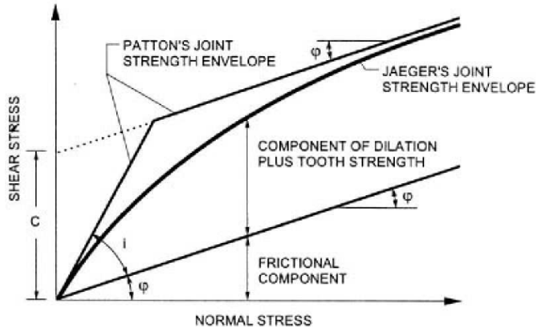
Fig. 2. Comparing the rock joint strength envelopes (Patton's bilinear model and Jaeger's strength envelope)
