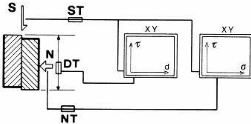
Fig. 4. Schematic diagram of the test monitoring arrangement (Tisa and Kovári, 1984).
