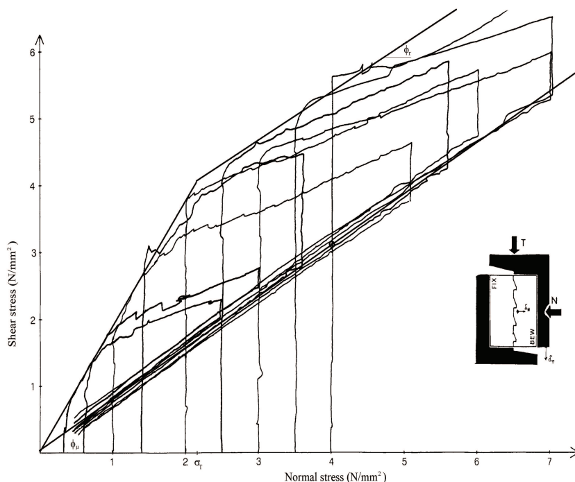
Fig. 5. Measured shear-stresses as functions of the continuously increasing normal stress
