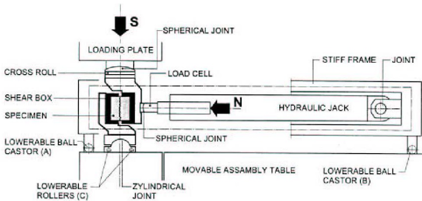
Fig. 3. Schematically view of the shear apparatus used in combination with a loading machine [7]
