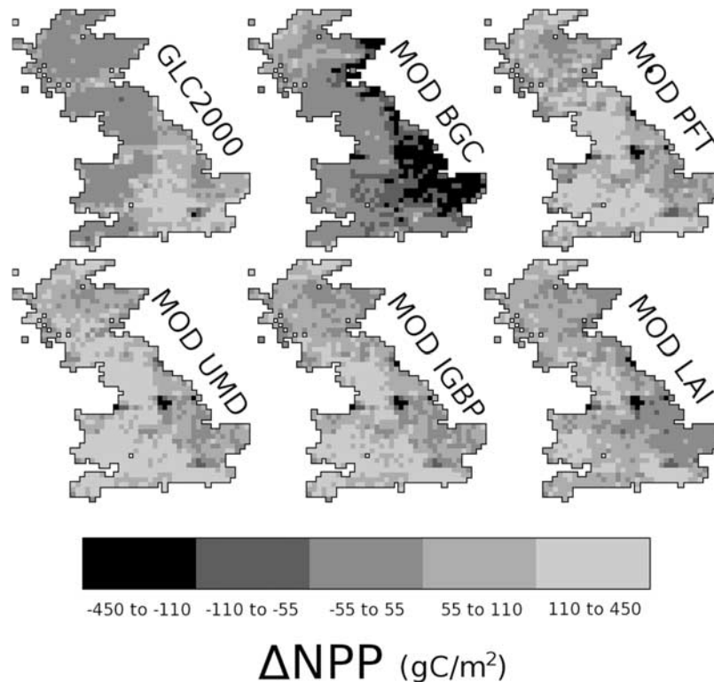
Figure 3b. Differences between Net Primary Production (NPP) predicted using LCM2000 and the other land cover products. Dark (light) areas indicate under (over)-prediction with respect to LCM2000. From the top left, moving clockwise the land cover classification used is GLC2000, MODIS-BGC, MODIS-PFT, MODIS LAI/fAPAR, MODIS IGBP and MODIS UMD.
