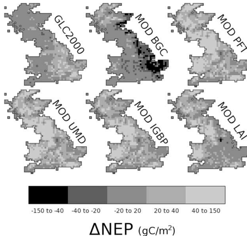
Figure 3c. Differences between Net Ecosystem Production (NEP) predicted using LCM2000 and the other land cover products. Dark (light) areas indicate under (over)-prediction with respect to LCM2000. From the top left, moving clockwise the land cover classification used is GLC2000, MODIS-BGC, MODIS-PFT, MODIS LAI/fAPAR, MODIS IGBP and MODIS UMD.
