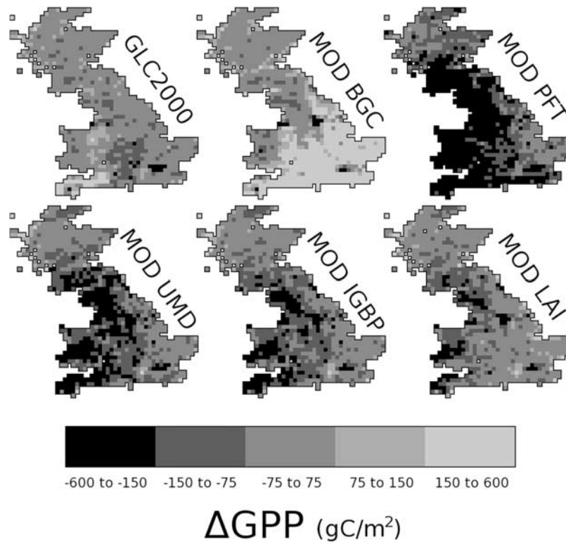
Figure 3a. Differences between Gross Primary Production (GPP) predicted using LCM2000 and the other land cover products. Dark (light) areas indicate under (over)-prediction with respect to LCM2000. From the top left, moving clockwise the land cover classification used is GLC2000, MODIS-BGC, MODIS-PFT, MODIS LAI/fAPAR, MODIS IGBP and MODIS UMD.
