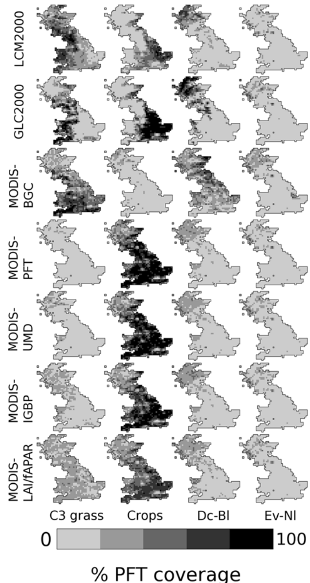
Figure 1. Proportions (from left to right) of the C3 grass, crop, deciduous broadleaf and evergreen needleleaf Plant Functional Types (PFTs) across Great Britain according to (a) LCM2000 (b) GLC2000 (c) MODIS-BGC (d) MODIS-PFT (e) MODIS-UMD (f) MODIS-IGBP (g) MODIS-LAI/fAPAR.
