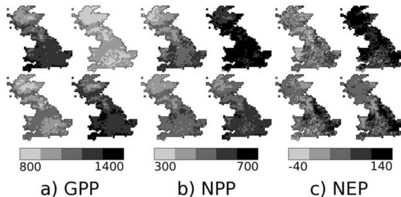
Figure 2. Estimated carbon fluxes for the year 2000 ( \text{gCm}^{-2} \text{a}^{-1} ) assuming Great Britain is entirely covered by C3 grasses, crops, evergreen needleleaf and deciduous broadleaf; clockwise from top left in each case.
