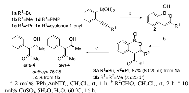
Scheme 1 Gold catalysed boron enolate formation/aldol reaction.
