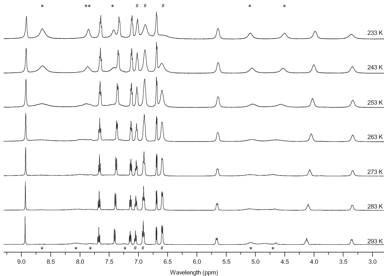
Fig. 6 VT ^1\text{H} NMR spectra of [\text{FeL}^2_3\text{Cu}](\text{ClO}_4)_2 in d_3\text{-acetonitrile} (* \text{OCH}_2\text{Py} , # Ph ).
