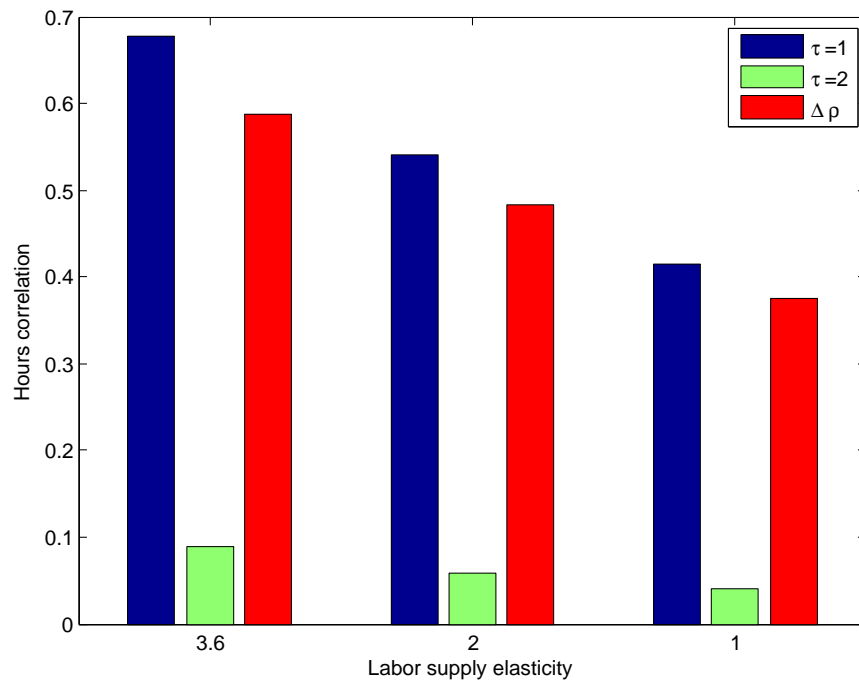
Figure 2: Trade and Synchronization: Two-Country Example
