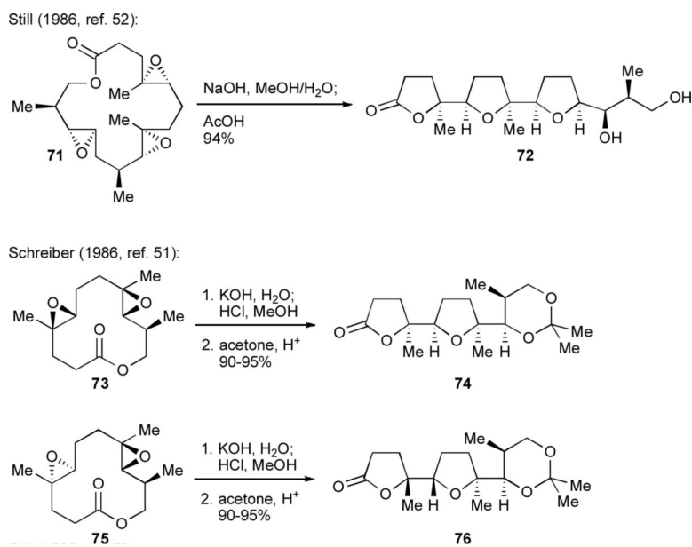
Scheme 15. Exo -selective cascades applied to the synthesis of subunits of monensin.
