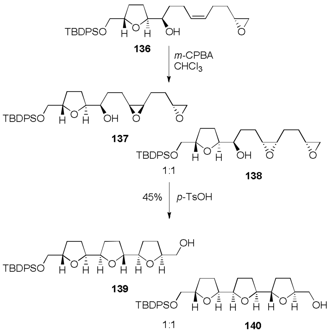
Scheme 15. Synthesis of tricyclic ionophores 139 and 140 via cascade of epoxide openings (Koert, 1994). [208]
