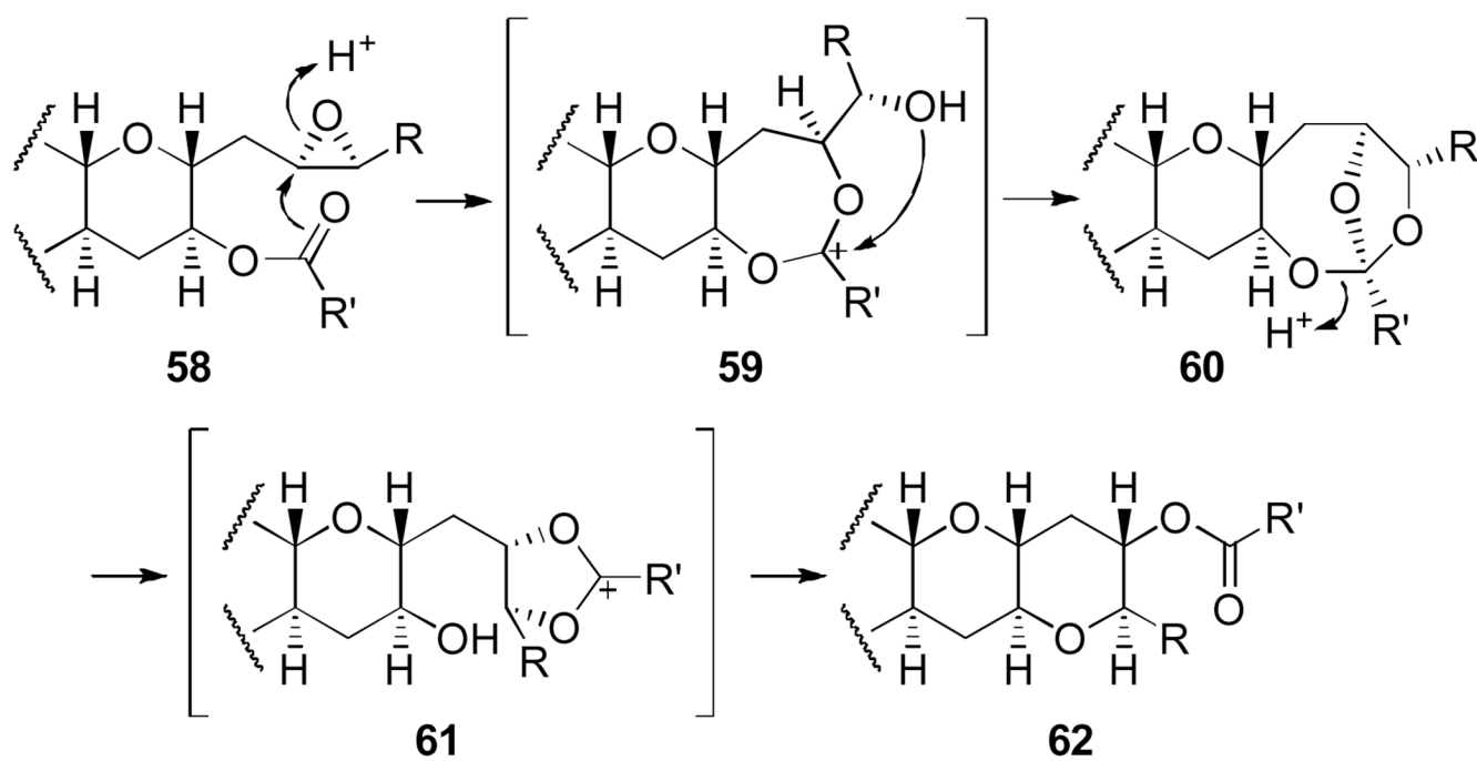
Figure 9. Biosynthesis of ladder polyethers via epoxy ester pathway (Giner, 2003).[166]
