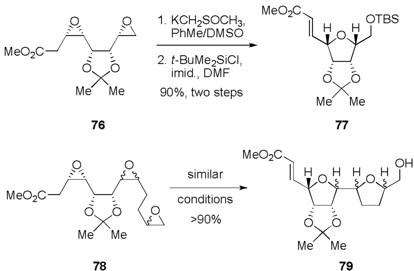
Scheme 5. Construction of the central backbone of aurodox and related epoxide-opening cascade leading to 2,5-linked bistetrahydrofuran 79 (Nicolaou, 1985).[189]
