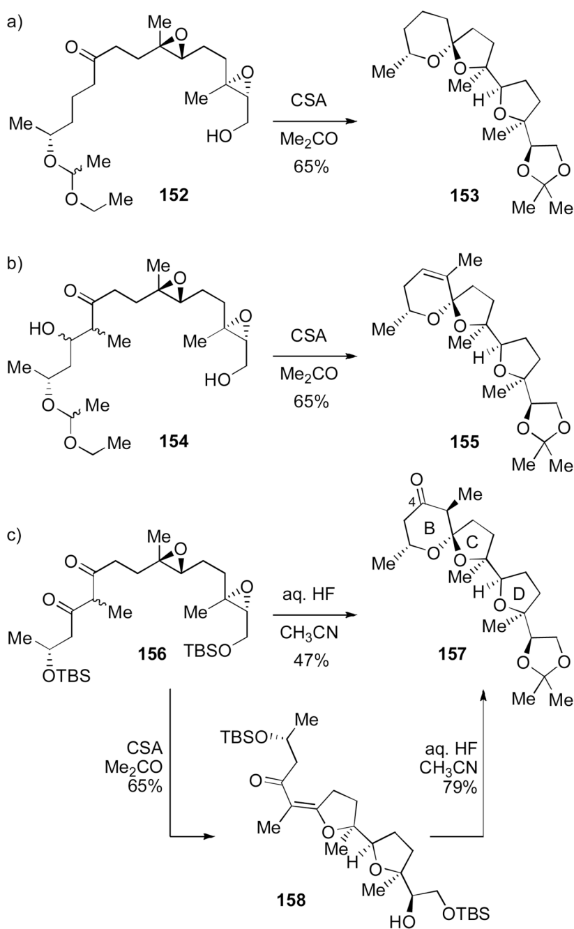
Scheme 18. Second and third-generation cascade approach to etheromycin (Paterson, 1988, 1989).[210, 211]
