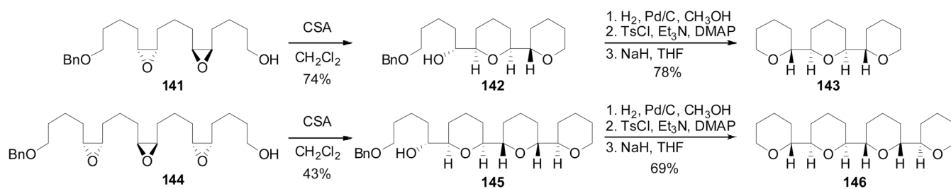
Scheme 16. Synthesis of oligotetrahydropyran ionophores 143 and 146 (Still, 1989).[209]
