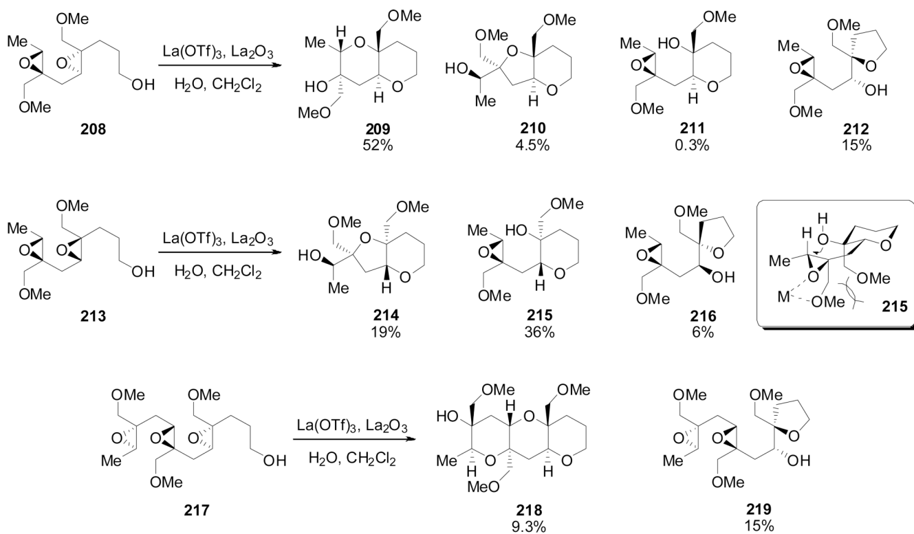
Scheme 30. Epoxide–opening cascades directed by methoxymethyl group (Murai, 2000).[238]
