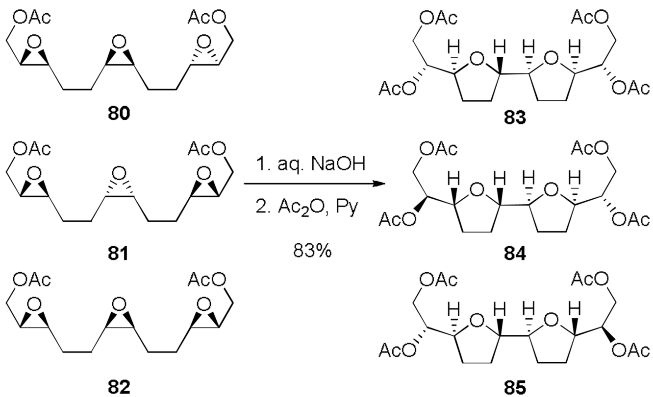
Scheme 6. Epoxide–opening cascades leading to formation of adjacent bistetrahydrofurans (Hoye, 1985). [190,191]
