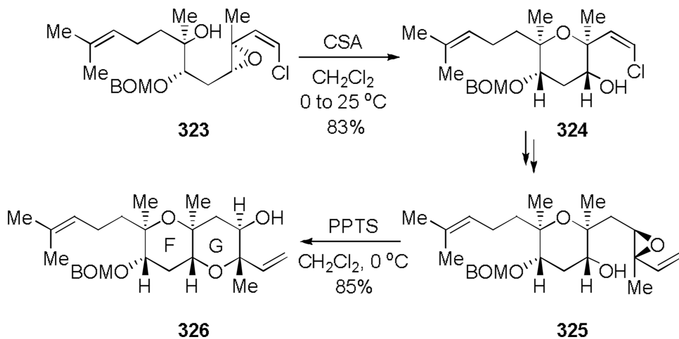
Scheme 44. Iterative synthesis of FG fragment of brevetoxin B (Nicolaou).[247]
