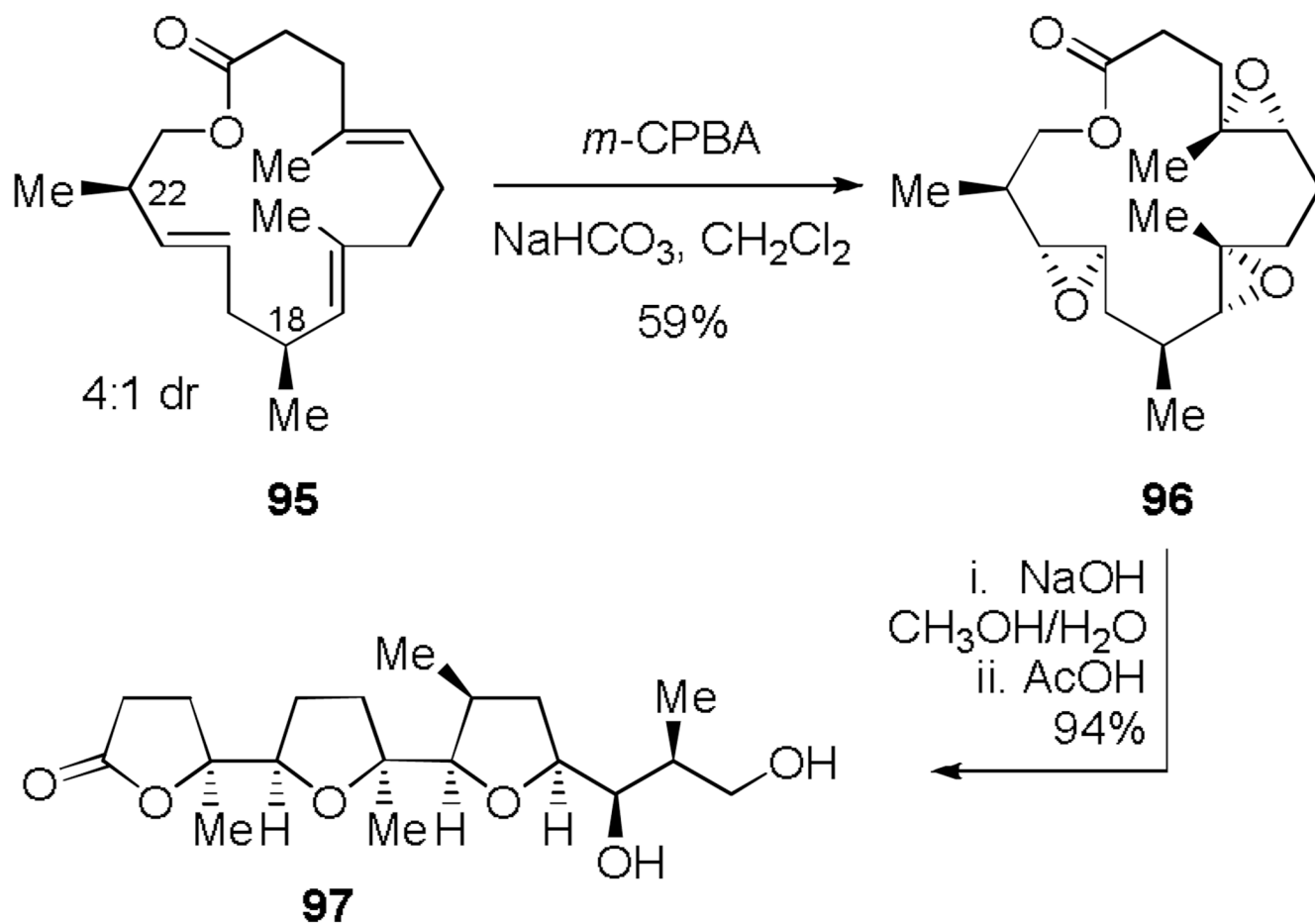
Scheme 9. Preparation of triepoxide 96 and epoxide-opening cascade leading to tricyclic product 97 (Still, 1986).[194]
