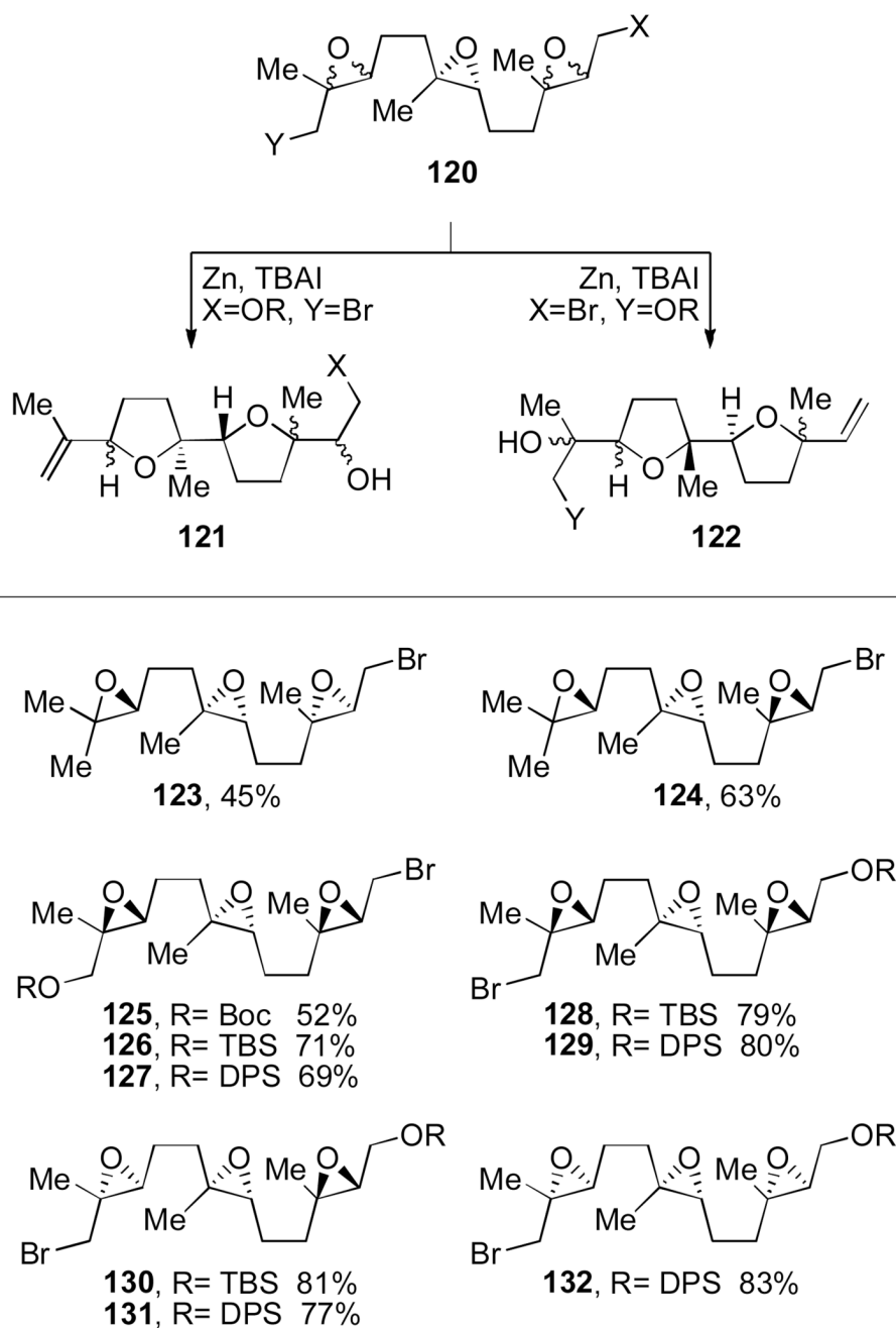
Figure 11. The synthesis of bistetrahydrofurans via epoxide-opening cascades of the triepoxyfarnesyl bromides (Marshall, 2008).[203,205]
