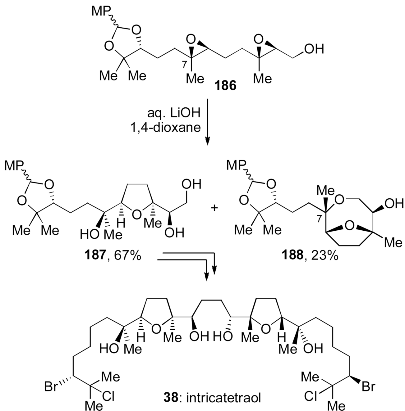
Scheme 26. Synthesis of C_5 -symmetric intricatetraol via epoxide-opening cascade/dimerization protocol (Morimoto, 2007).[227]
