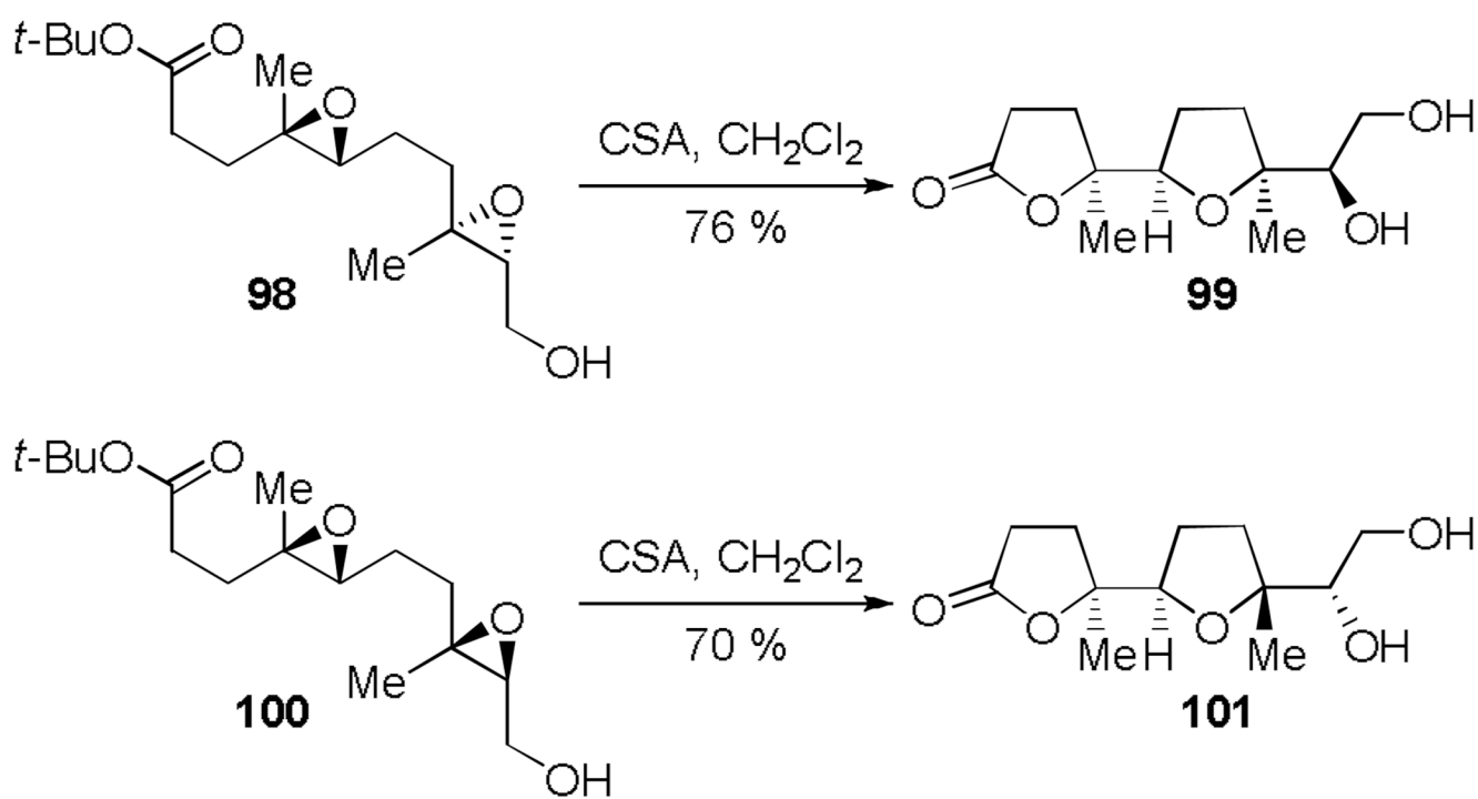
Scheme 10. Epoxide-opening cascades reported by Paterson (1987).[197]
