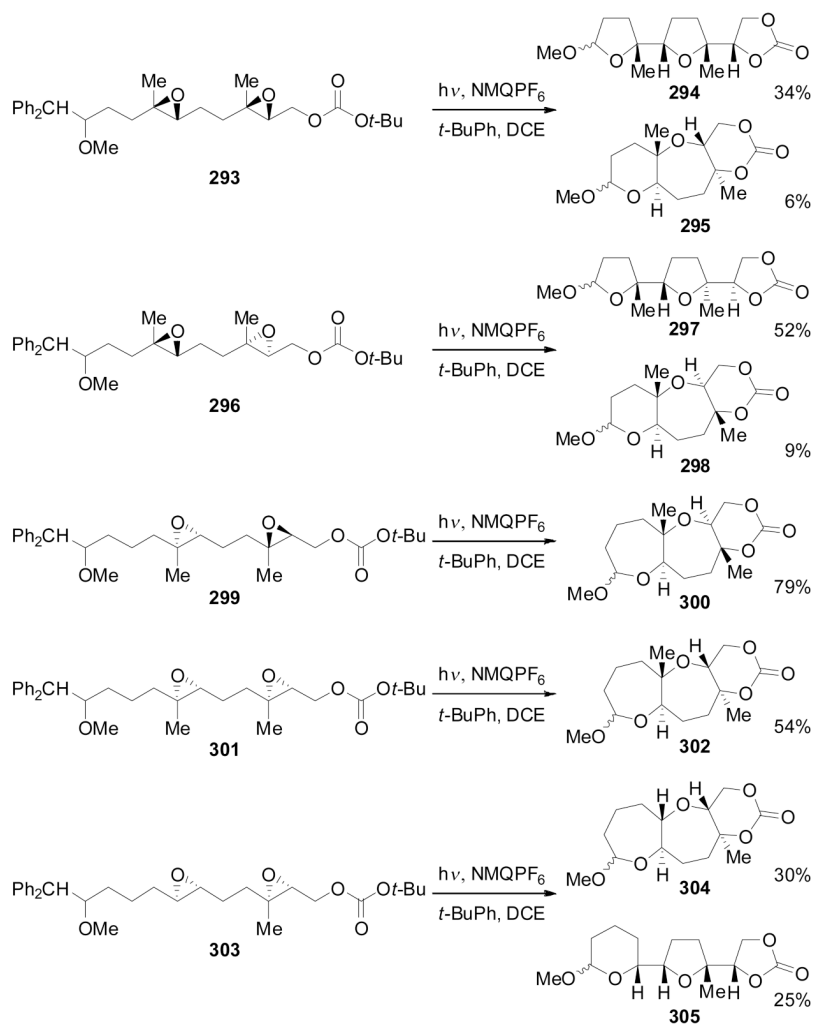
Scheme 40. Epoxide-opening cascades initiated by oxidative cleavage of homobenzylic ethers (Floreancig, 2007).[244]
