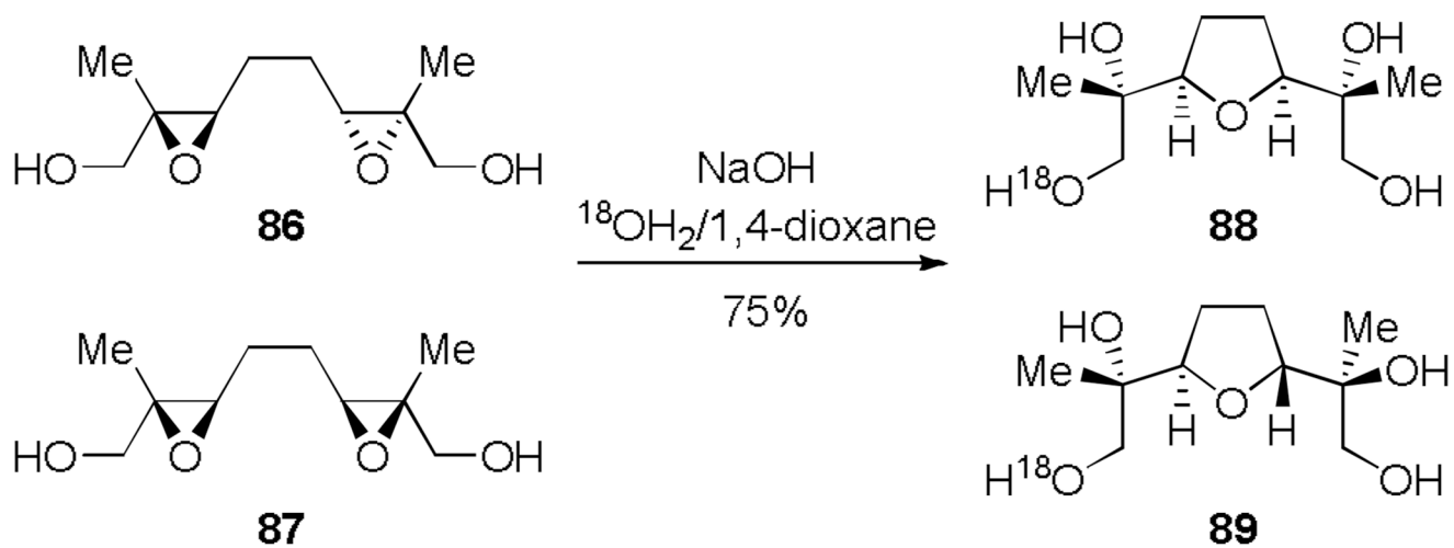
Scheme 7. Studies supporting the Payne rearrangement mechanism in epoxide–opening cascades (Hoye, 1987).[192]
