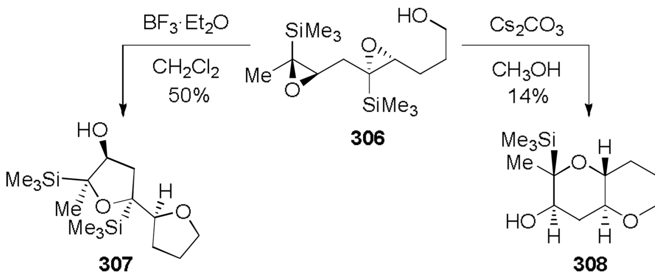
Scheme 41. Silyl directed cascade cyclizations of epoxysilanes (Jamison, 2006).[245]
