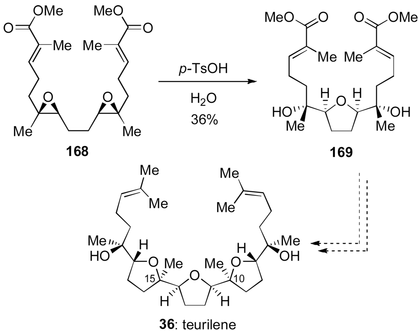
Scheme 21. Synthesis of teurilene core via epoxide-opening cascade (Lindel, 1995).[214]
