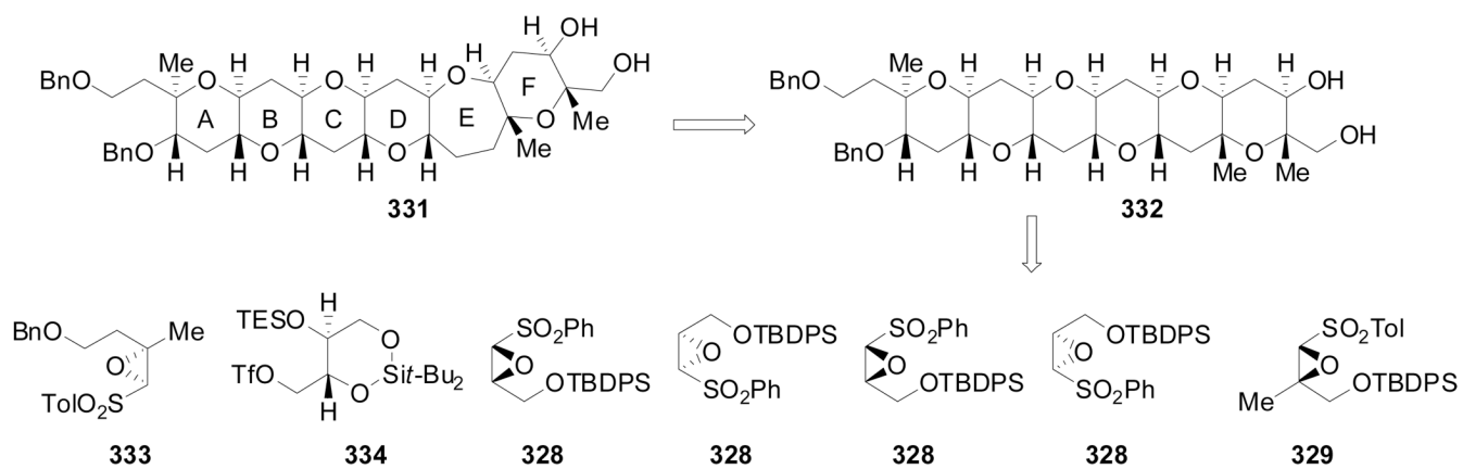
Figure 14. Conceptual retrosynthesis of the ABCDEF ring fragment of yessotoxin and adriatoxin (Mori, 2003).[285]
