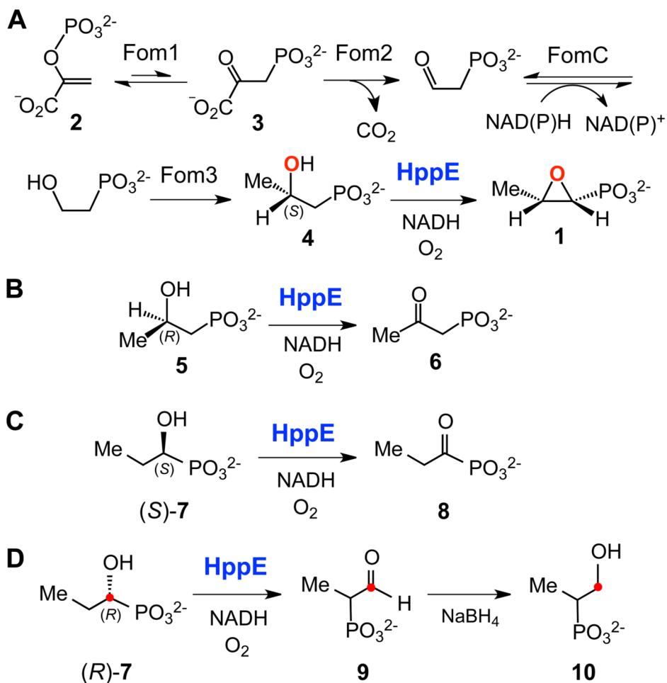
Figure 1. Fosfomycin biosynthetic pathway and HppE-catalyzed conversion of various substrate analogues
