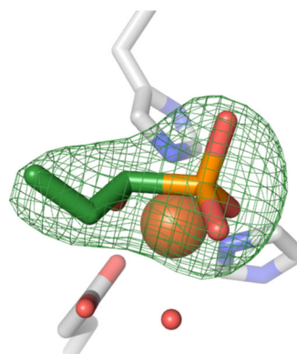
Figure 3. Structures of (S)-7 and (R)-7 bound to the iron center of HppE in a bidentate mode (A) (S)-7 (carbons in blue) in F_o-F_c omit map density contoured at 6\sigma (left) and its chemical structure (right), with hydrogen atoms accessible for abstraction in red and inaccessible in blue. The putative dioxygen binding site on Fe is partially occupied by water molecules (red spheres) in both of these structures (Fe-H 2 O distances are 3.7 and 3.0 Å). Colors: Fe in rust, P in orange, O in red, N in blue, protein C in gray. (B) (R)-7 (carbons in green) in F_o-F_c omit map density contoured at 6\sigma (left) and its chemical structure (right). Hydrogen atoms labeled as in (A).
