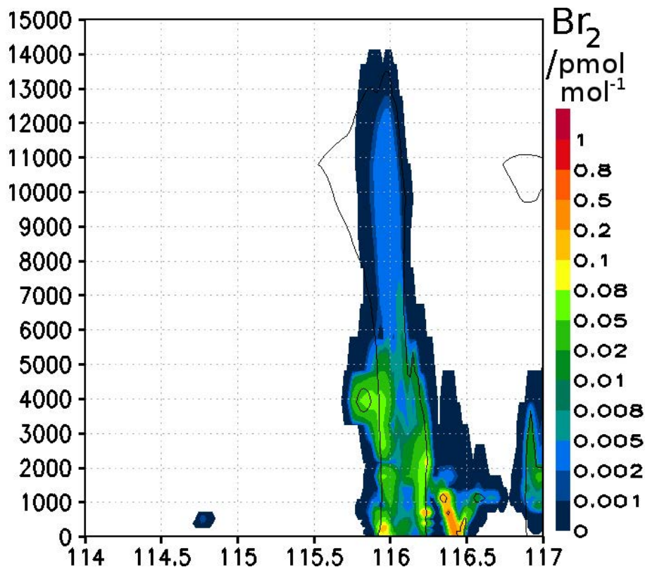
Fig. 18. Simulated vertical cross sections of \text{Br}_2 across a latitude of 5^\circ 30' \text{ N} during the peak of convective activity at Region 2B at 16:00 LT.
