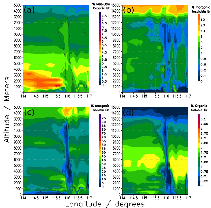
Fig. 17. Simulated vertical cross sections of the relative contributions of various bromine containing species to the total bromine atom budget across a latitude of 5^{\circ}30'N during the peak of convective activity at Region 2B at 16:00 LT. Figure (a) shows the relative contribution from bromine atoms present as insoluble organic bromine, (b) shows the relative contribution from inorganic insoluble, (c) the relative contribution from inorganic soluble, and (d) the relative contribution from organic soluble bromine. Note that the dissolved HBr and HOBr as not included in the calculation of any of the budgets shown here. The y-axis shows the altitude in meters and the x-axis shows the longitude.
