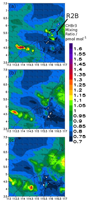
Fig. 12. Simulated CHBr 3 mixing ratios at 12 km on 19 November during a portion of Flight B showing the lofting of CHBr 3 and its transport from Region 2B to the West. Plot (a) is from 16:00 LT, plot (b) from 17:00 LT, and plot (c) from 18:00 LT. The convective event that lofted CHBr 3 at Region 2B in this figure is the same event shown in Fig. 11. The y-axis shows the latitude and the x-axis shows the longitude. The wind vectors at 12 km are shown in addition to the the location of Region 2B.
