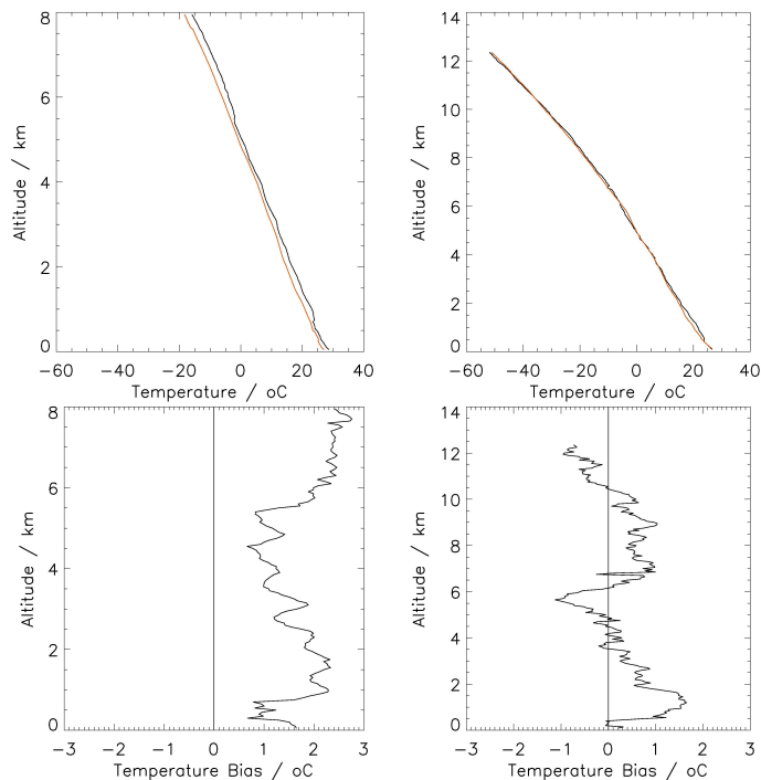
Fig. 9. Comparison between the average observed temperature vertical profiles during both Flights A and B and the model output interpolated to the aircraft track. The left hand figures show the comparison with Flight A, and the right hand figures the comparison with Flight B. The back line shows the sonde observation data and the orange line shows the model data. Flight A was compared to the secondary model grid (spatial resolution 10km × 10km), and Flight B to the finest model grid (spatial resolution 2km × 2km).
