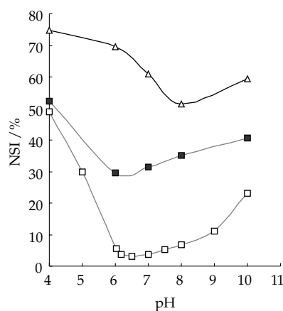
Fig. 5. Nitrogen soluble index of GHP- \lambda C conjugate -□, control; -■-, gluten hydrolysate; -△-, GHP- \lambda C conjugate. The preparation condition of the conjugate: pH=10.0, GHP/ \lambda C ratio=6:1, reaction time=10 days, reaction temperature=70 °C
