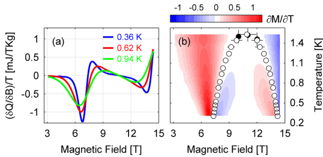
FIG. 4 (color online). Magnetocaloric effect in (\text{Hpip})_2\text{CuBr}_4 . (a) Heat-flow \delta Q to and from the sample as a function of magnetic field divided by temperature, (\delta Q/\delta B)/T . (b) Contour plot of \partial M/\partial T as a function of field and temperature. White circles denote the phase boundary derived from \partial M/\partial T = 0 (see also Fig. 1), while black circles are maxima in the specific heat, \partial C_m/\partial T = 0 , obtained at fixed field.
