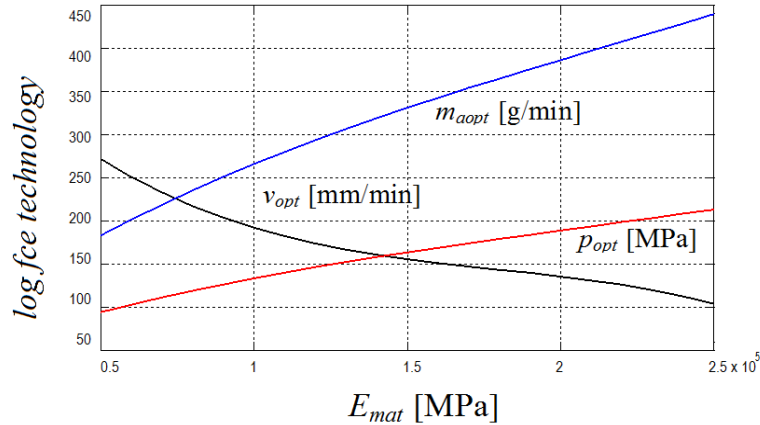
Fig.5a. Optimized technological parameters according to E_{mat} [MPa] according to the above-presented (13), (14) and (15).
