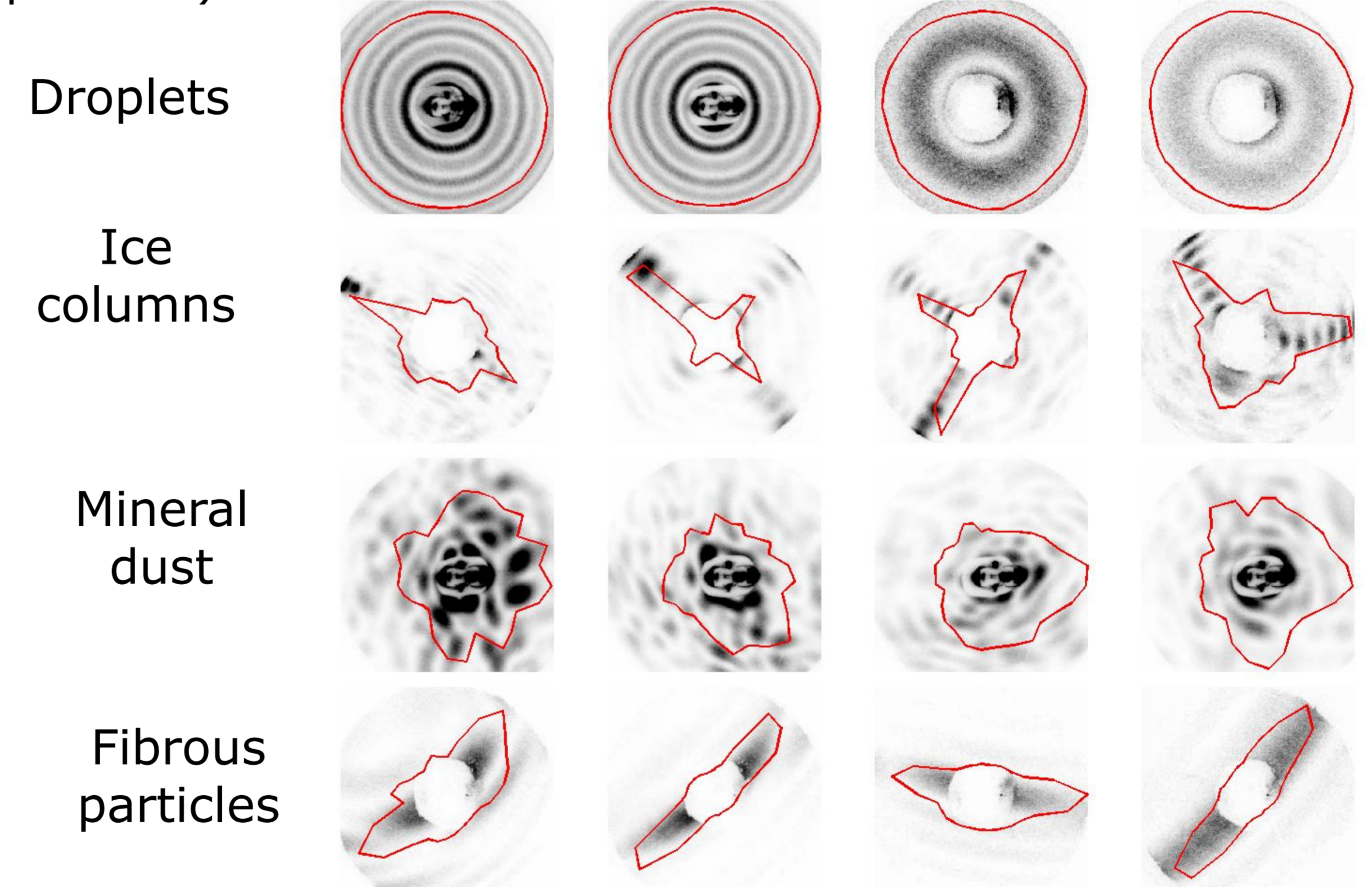
Fig.4: Examples of particle data captures by the SID2 (red line) and SID3 (2D-images) probes. The APC will combine both techniques to yield detailed morphological data from large number of individual particles down to micrometre sizes.
