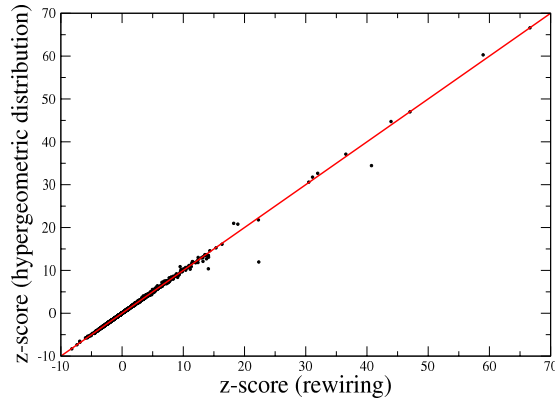
Figure 5. Scatter plot of the z-scores based on 1000 rewiring experiments versus the z-scores obtained with the probabilistic modeling, for the 3-maintenance period from 24-Dec-2004 to 23-Mar-2005.
