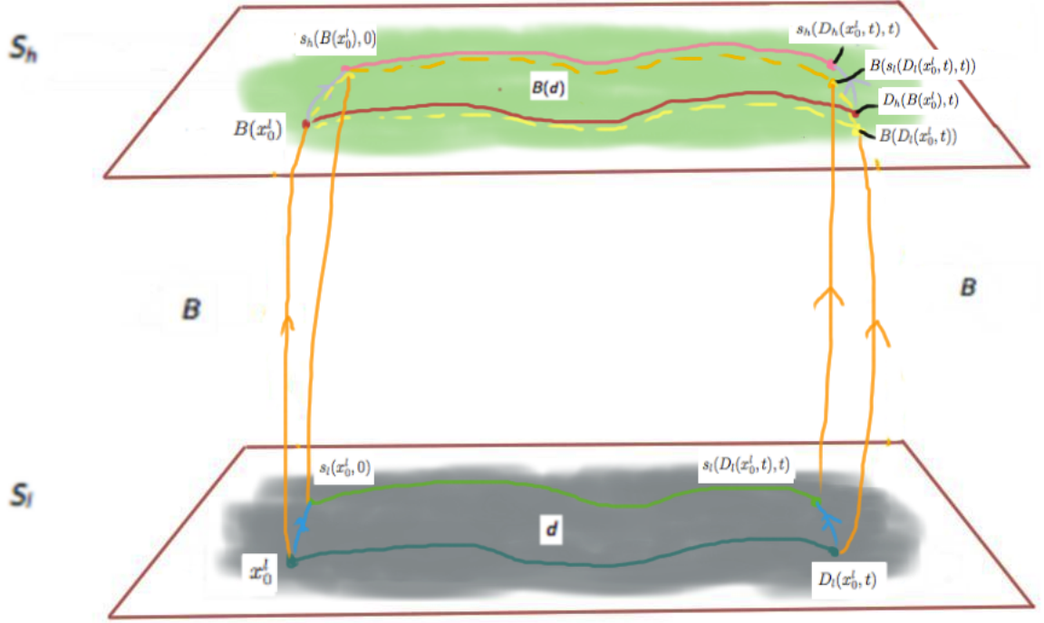
Figure 2: The symmetry condition of DS reduction entails that if two D_h -trajectories lying in B(d) are related by a high-level symmetry, then there is a corresponding low-level symmetry relating the two low-level trajectories that approximate these high-level trajectories under the bridge map.
