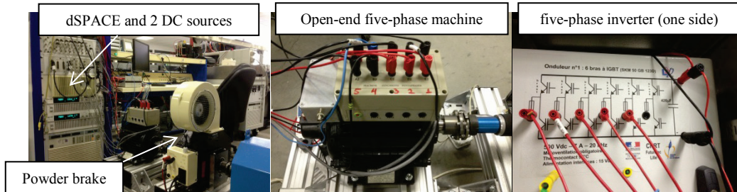
Figure 7 : Laboratory experimental platform setup
