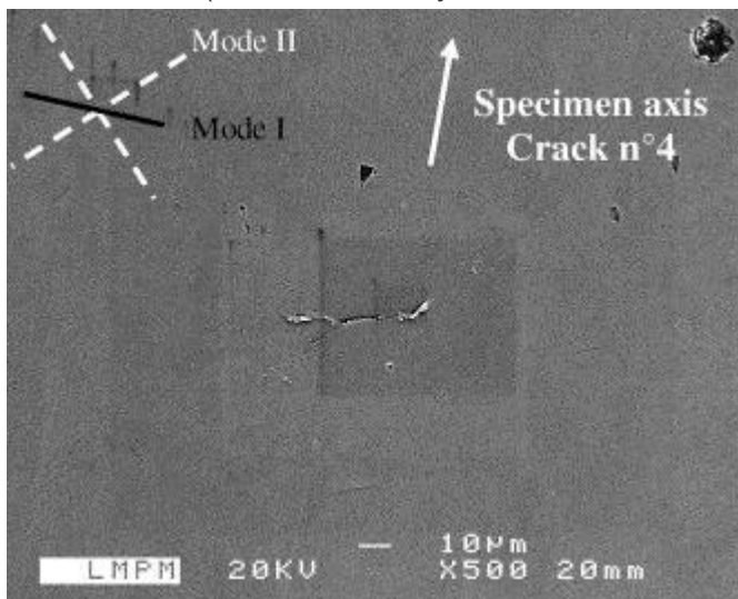
Fig. 7. SEM view of the crack No. 4 On the sample C36TR05 after 2 \times 10^6 cycles.
