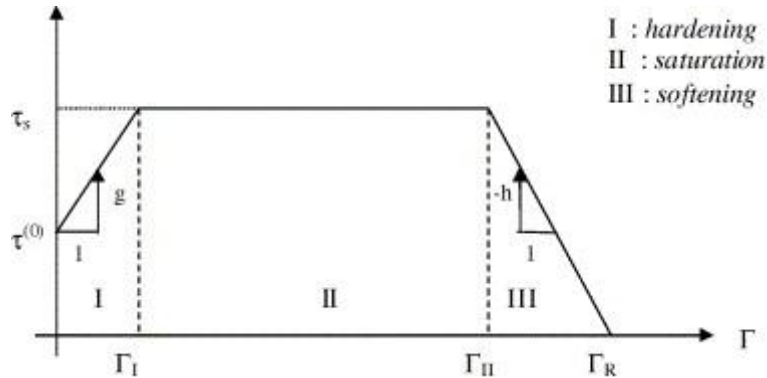
Fig. 2. Diagrammatic representation of the construction of the three plastic behavior proposal [1].
