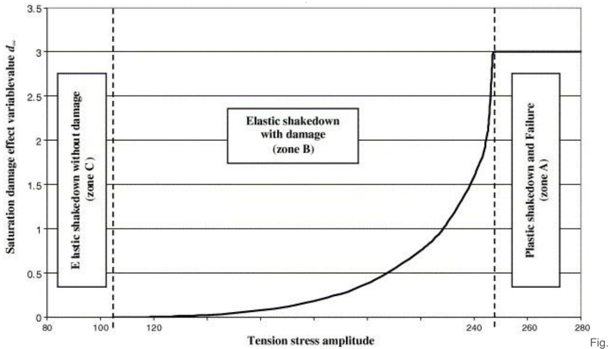
27. Saturation damage effect variable d_s according to constant stress amplitude of the tension loading.
