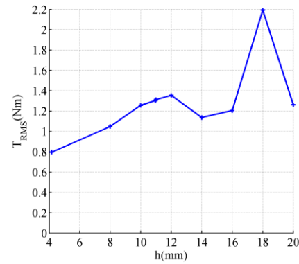
b. RMS value of cogging torque for different magnet configurations.
