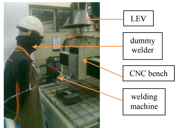
Fig. 1 Experimental set-up during standing position
