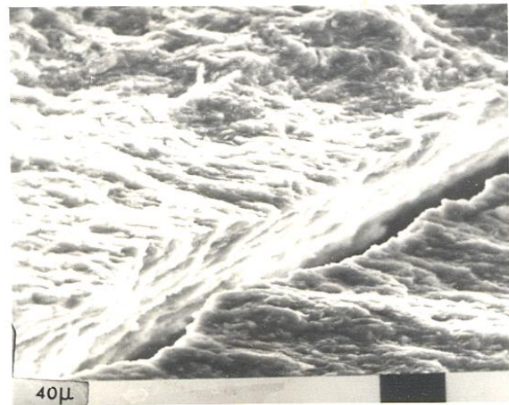
Fig. 5 – Scanning Electron Micrograph of preferential orientation of clay particles initially along drainage channels dissipating excessive pore water pressures. [9]
