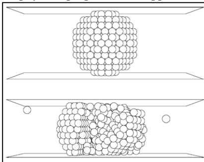
Fig. 10 Agglomerated modeling crushable grains [20]
