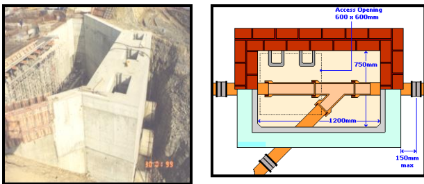
a) Intake tower Power Station Domestic manhole
