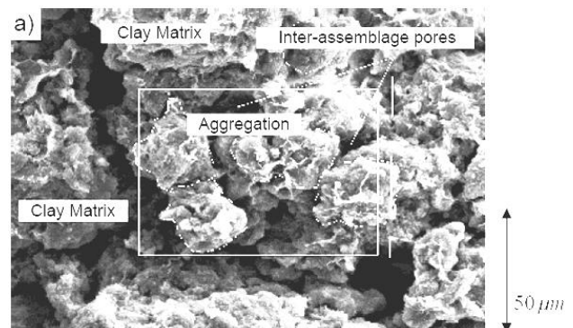
Fig. 8 Clay matrix, aggregation and inter assemblage pores
