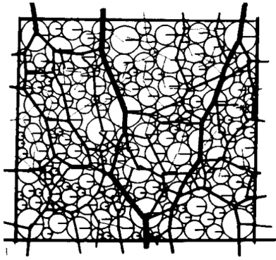
Fig. 9 Stress as a network of contact forces [12]
