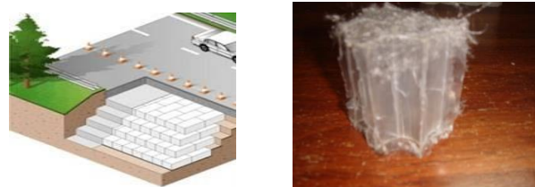
Fig. 13 a) use of EPS blocks b) view of a GCM
