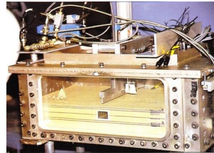
b) Complex instrumentation within the 400x600x200mm strong sample box.
