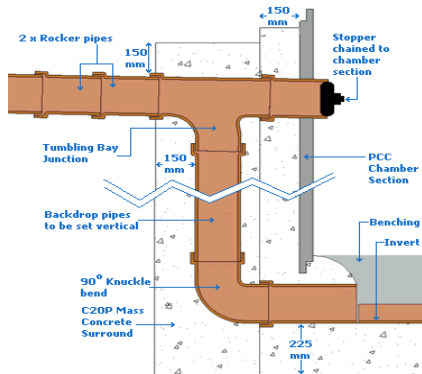
b) Provision of rocker pipes at vulnerable pipe joints
