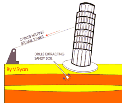
Fig 3. Soil Extraction Technique for Restoration of Tower of Pisa [7]
