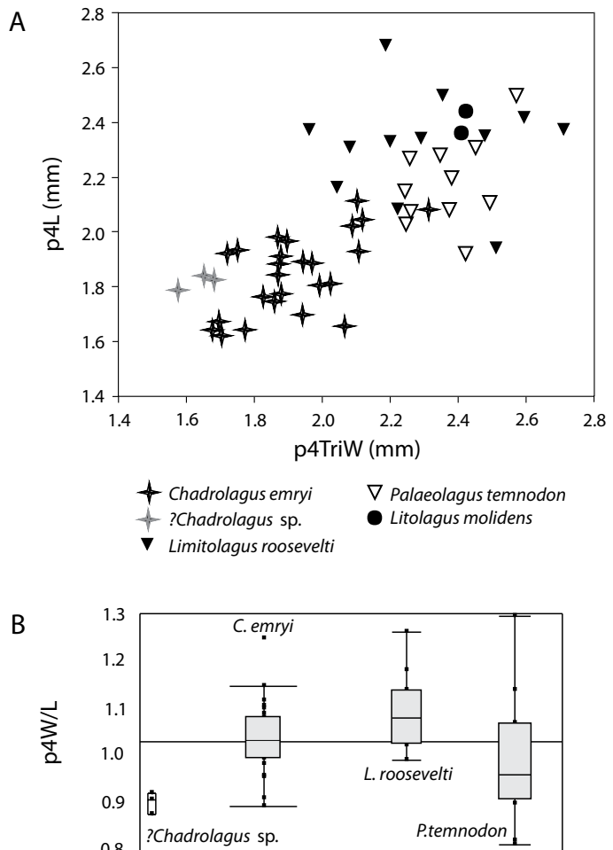
FIG. 17. Proportions of p4 in ? Chadrolagus sp. from the Pipestone Springs area, compared with morphologically closest lagomorph species from the middle Chadronian–early Orellan interval. A , scatter-plot of the tooth length (p4L) to the trigonid width (p4TriW) ratio; B , box plot of this ratio.
