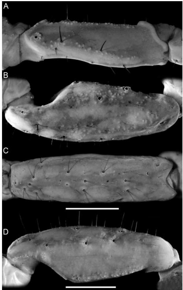
FIGURE 16. Urophonius tregualemuensis Cekalovic, 1981, \sigma (AMNH), dextral pedipalp segments. A. Femur, dorsal aspect. B. Patella, dorsal aspect. C. Patella, external aspect. D. Patella, ventral aspect. Scale bar = 1 mm.
