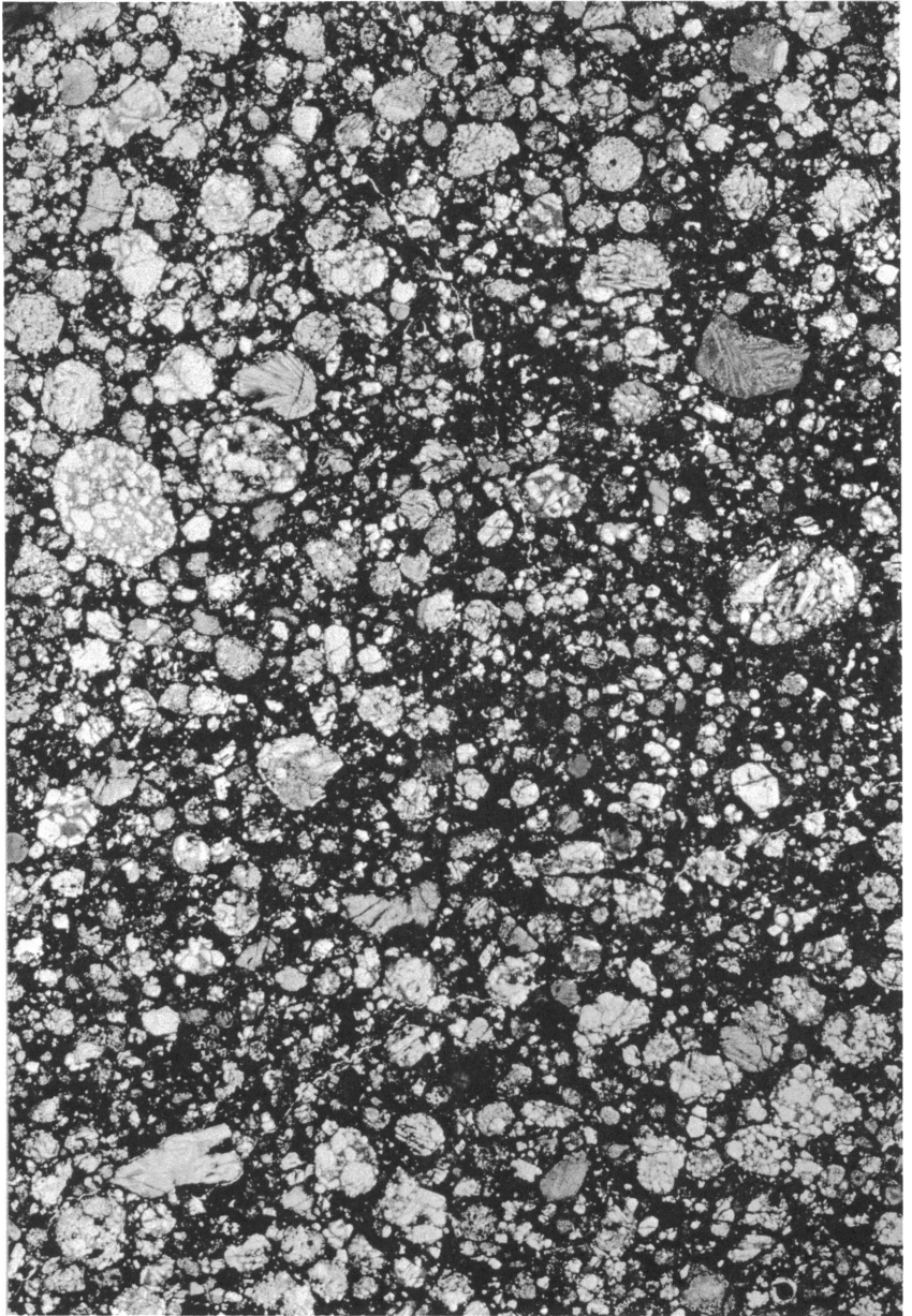
FIG. 1. Photomicrograph of the Selma meteorite. Chondrules of granular olivine and fibrous and prismatic hypersthene in an opaque ground mass. The largest chondrule is 1.5 mm. in diameter.
