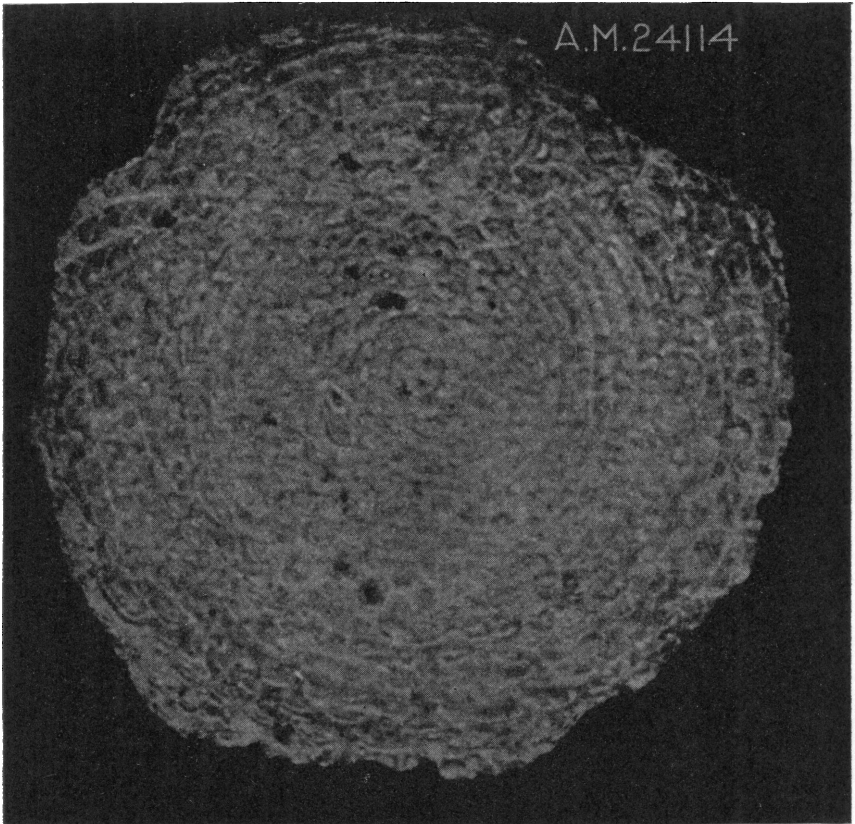
Figure 9.—Horizontal section of Omphalocyclus macropora (Lamarck). \times 30 . American Museum No. 24,114.
