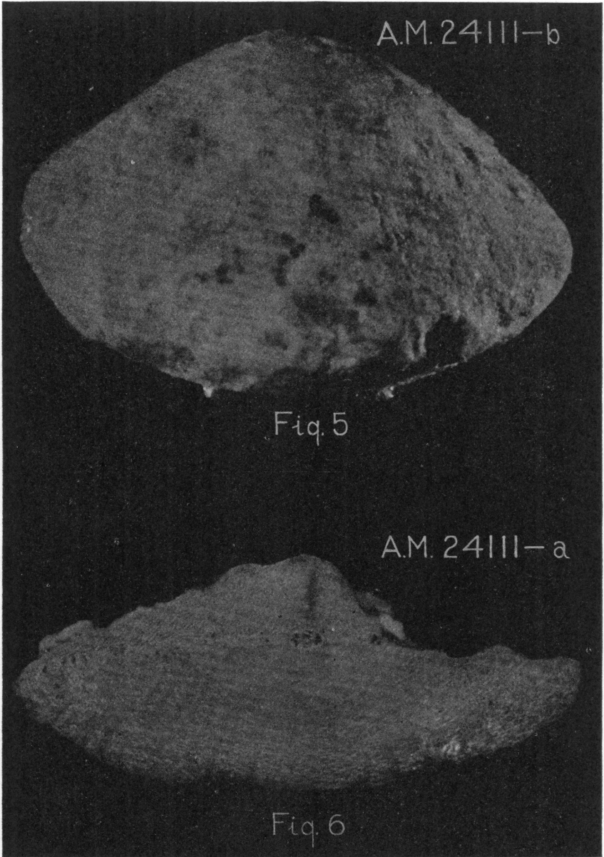
Figure 5.—External view of Gallowayina browni , new genus, new species. \times 15 . American Museum No. 24,111-b.
