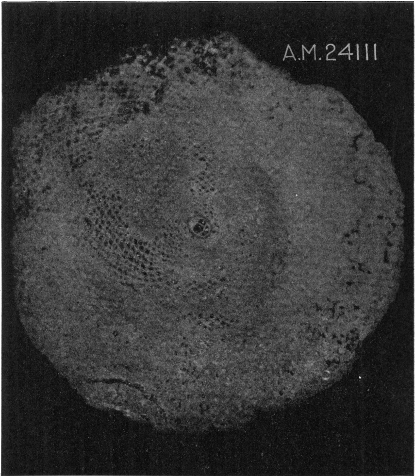
Figure 7.—Horizontal section of Gallowayina browni , new genus, new species. \times 15 . American Museum No. 24,111.
