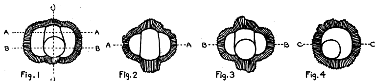
Figure 1.—A horizontal section of the nucleoconch of Gallowayina browni , showing the four chambers. The dotted lines show the locations of the vertical sections in figures 2, 3 and 4.
